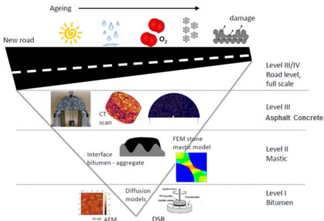
FIGURE 5: Example of an testing and modelling program aiming to account for local climate and mixture composition effects in aging (29)
