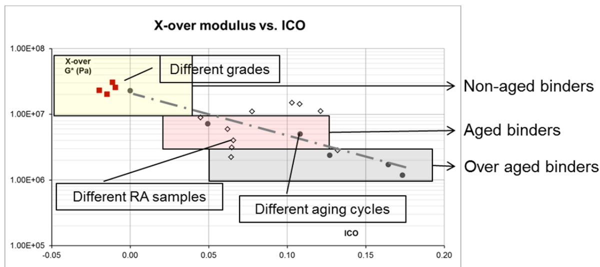
FIGURE 4: Chemical (carbonyl index) and rheological (cross-over modulus) properties of laboratory aged and field samples (28)
