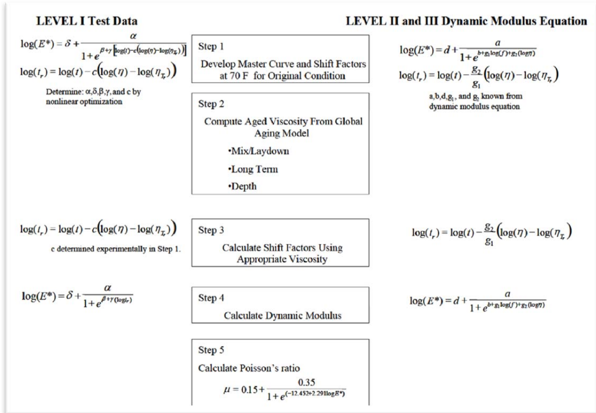
FIGURE 1 Aging of AC properties in the MEPDG works through regression based on bitumen aging (copy of fig 2.2.3 (13))
