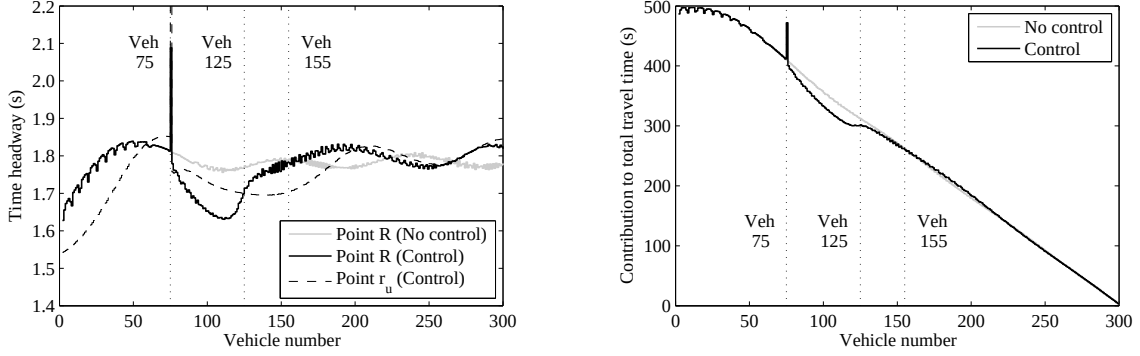
(a) Time headway of every vehicle at points r_u and R . Time headways at point R oscillate due to differences in speed profile between consecutive vehicles as they accelerate to the desired speed after exiting the sag.
