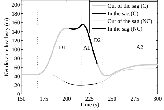
(d) Net distance headway of vehicle 75 over time in the scenario with M = \{75\} (C) and the no-control scenario (NC).
