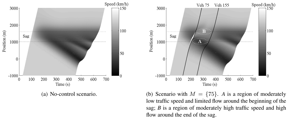
Figure 9: Speed contour plots of the no-control scenario and the control scenario with M = \{75\} .
