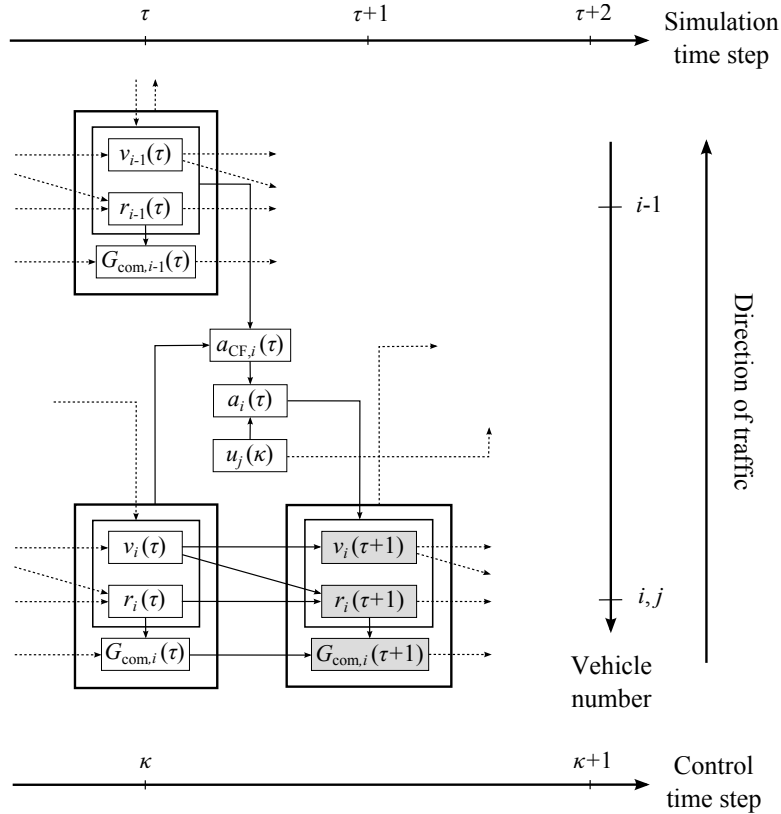
Figure 3: Overview of the inputs needed to calculate the state dynamics.
