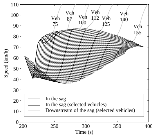
Figure 8: Effect of the DADA maneuver of the controlled vehicle on the behavior of the first 90 following vehicles in the control scenario with M = \{75\} .
