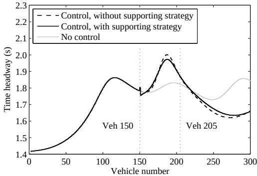
(c) Time headway of every vehicle at point r_d + 150 m.
