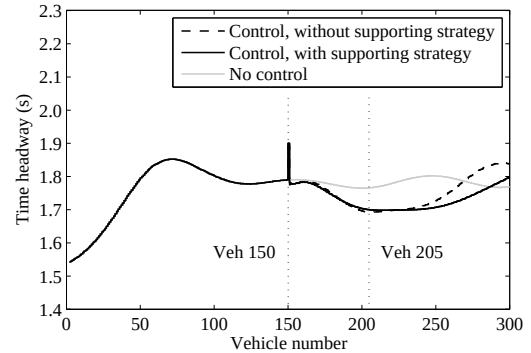
(d) Time headway of every vehicle at the end of the sag ( r_u ).
