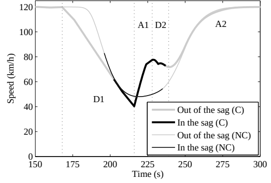
(b) Speed of vehicle 75 over time in the scenario with M = \{75\} (C) and the no-control scenario (NC).
