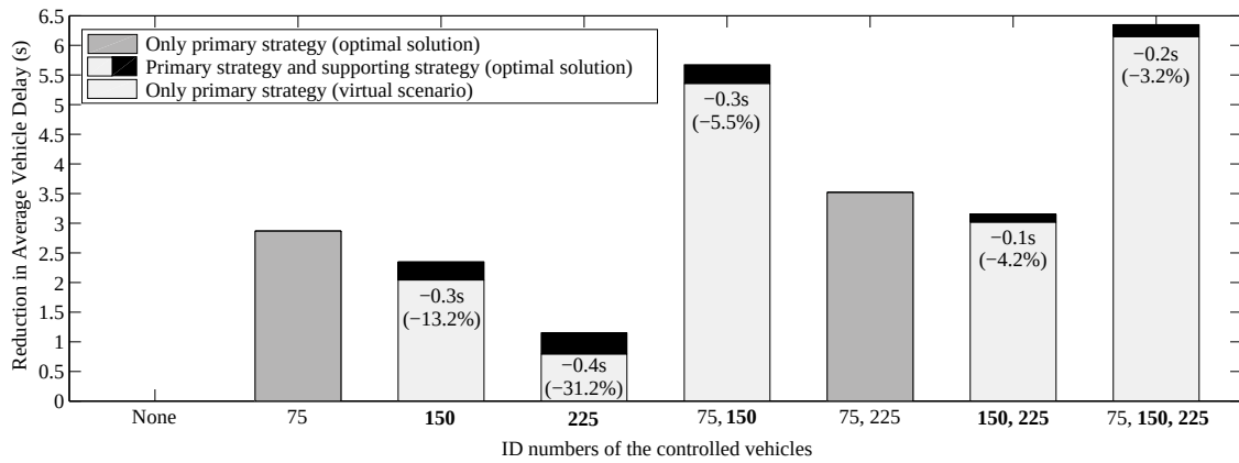
(b) Reduction in average vehicle delay (AVD) in every control scenario in comparison with the no-control scenario. In the horizontal axis, numbers in normal font indicate controlled vehicles that use only the primary strategy, whereas numbers in bold indicate controlled vehicles that use both the primary strategy and the supporting strategy. For the control scenarios in which controlled vehicles use the supporting control strategy, the figure also shows the AVD reduction in the corresponding virtual scenarios (in which the supporting strategy is not applied). For those scenarios, the numbers inside the bars indicate the absolute and relative difference in AVD reduction between the virtual scenario (without supporting strategy) and the control scenario with the optimal solution (which includes the supporting strategy).
