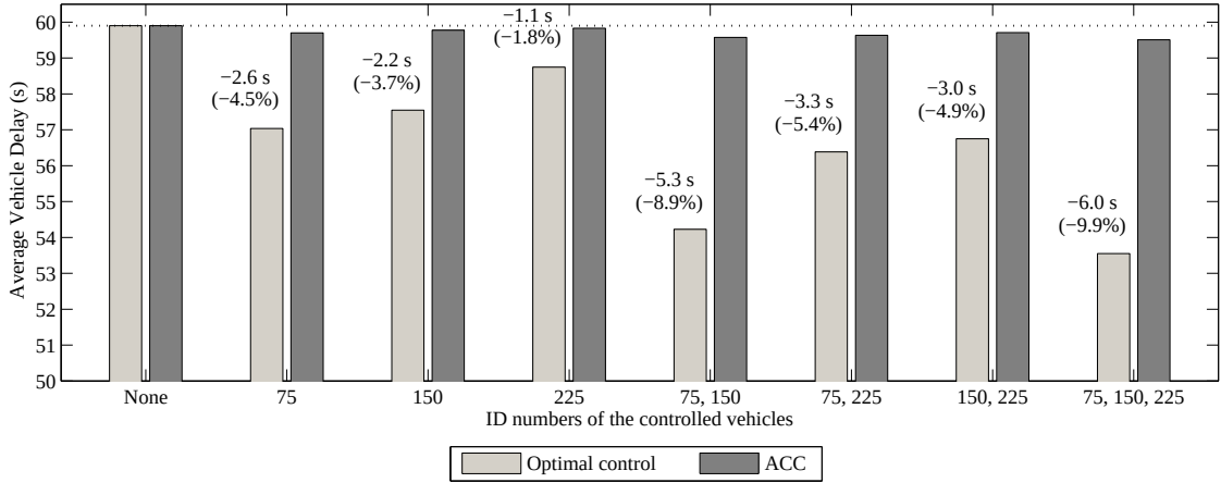
Figure 6: Average vehicle delay (AVD) in the no-control scenario, the optimal control scenarios and the ACC scenarios. The numbers on top of the light-gray bars indicate the difference in AVD and the difference in relative AVD reduction in comparison with the no-control scenario between the optimal control scenarios and the ACC scenarios with the same M .
