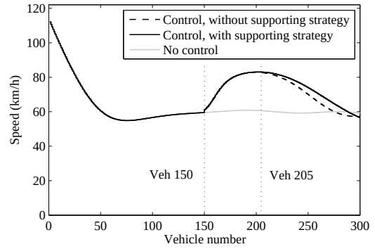
(b) Speed of every vehicle at the end of the sag ( r_u ).
