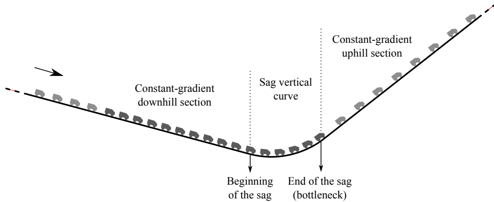
Figure 1: Freeway stretch with a sag: vertical profile and typical traffic conditions with high demand (light-gray vehicles are driving in free flow; dark-gray vehicles are driving in congested flow).
