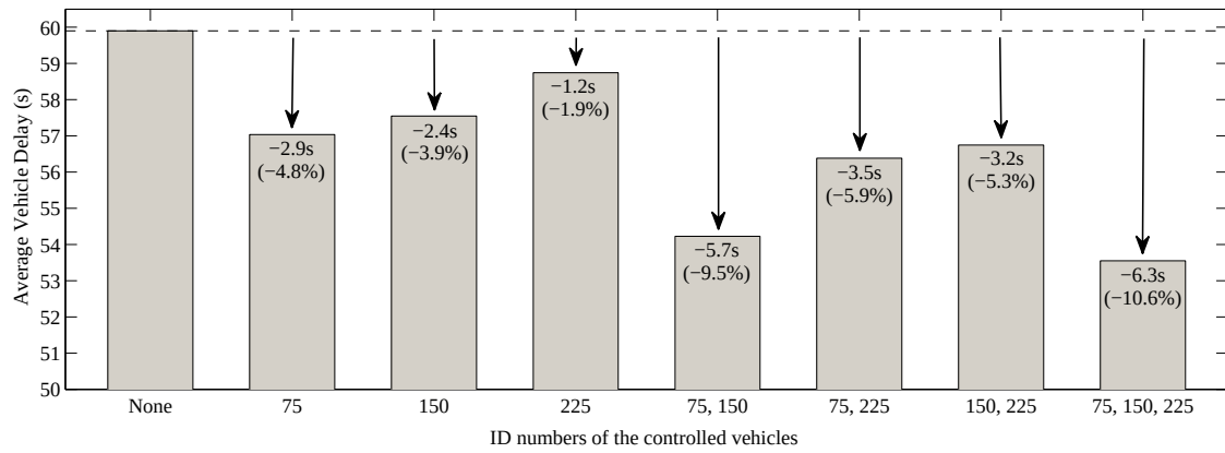
(a) Average vehicle delay (AVD) in every scenario. The numbers inside the bars indicate the absolute and relative difference in comparison with the no-control scenario.
