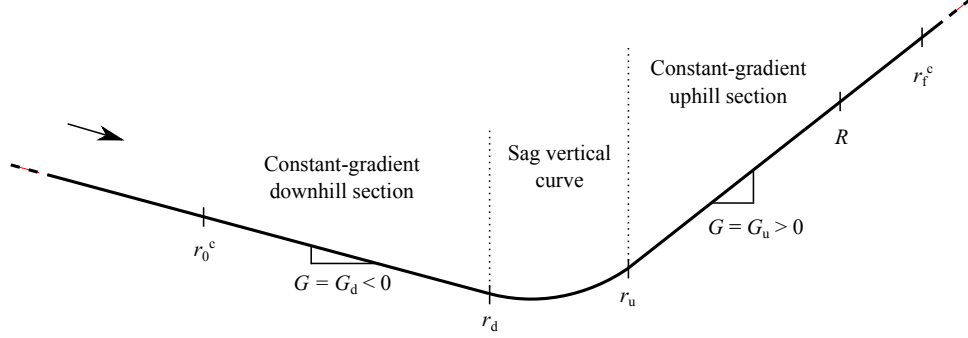
Figure 4: Vertical profile of the freeway stretch.
