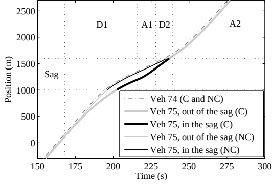
(c) Positions of vehicle 75 and its leader over time in the scenario with M = \{75\} (C) and the no-control scenario (NC).
