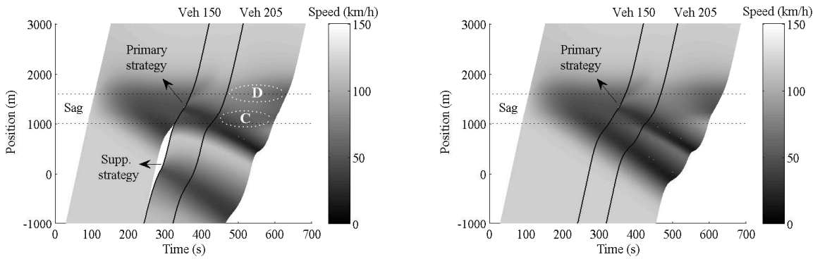
(a) Control scenario with M = \{150\} . C is a region located on the first part of the sag that has slightly lower speed and flow than in the virtual scenario; D is a region around the end of the sag that has slightly higher speed and flow than in the virtual scenario.
