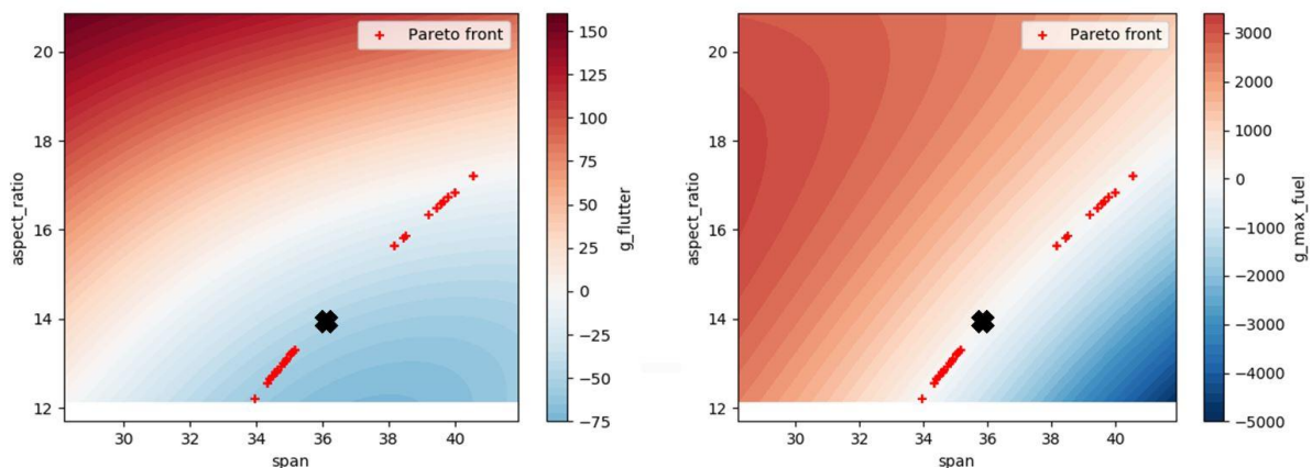
Fig. 12 flutter (left) and maximum fuel (right) contour plot using span and aspect ratio as design variables (baseline values represented by the black cross)
