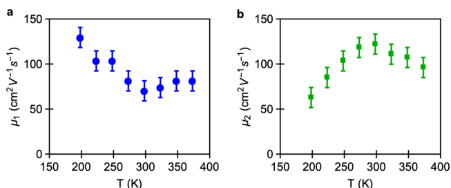
Figure 3. Temperature-dependent mobility for charges of type 1 and 2 in panel (a,b), respectively.
