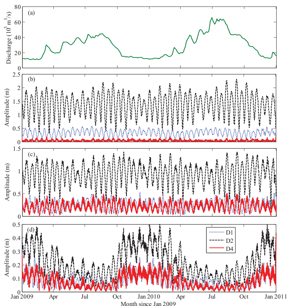
Figure 7. (a) River discharge at Datong; amplitudes of the diurnal ( D_1 ), the semidiurnal ( D_2 ), and the quarter-diurnal ( D_4 ) tides at (b) Niupijiao, (c) Xuliujing, and (d) Nanjing for 2009 and 2010, determined by CWT analyses.
