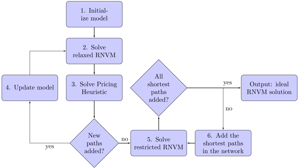
Fig. 4. Heuristic for generating new passenger paths.
