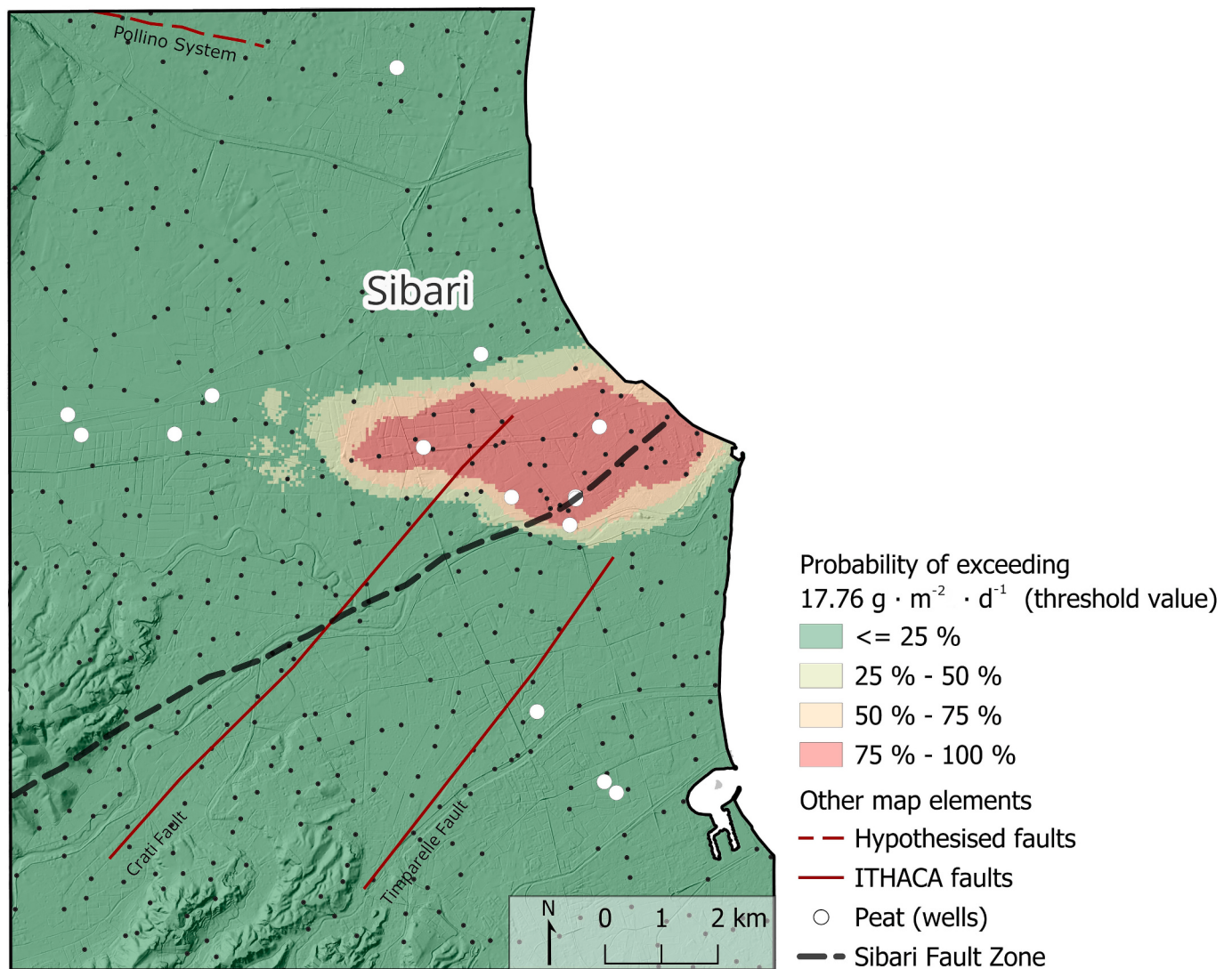
Fig. 5. Probability map of CO 2 flux created through the sequential Gaussian simulations and simple kriging as interpolation method. The map shows the probability that the measured value is greater than a threshold value, specifically 17.76 \text{ g} \cdot \text{m}^{-2} \cdot \text{d}^{-1} .
