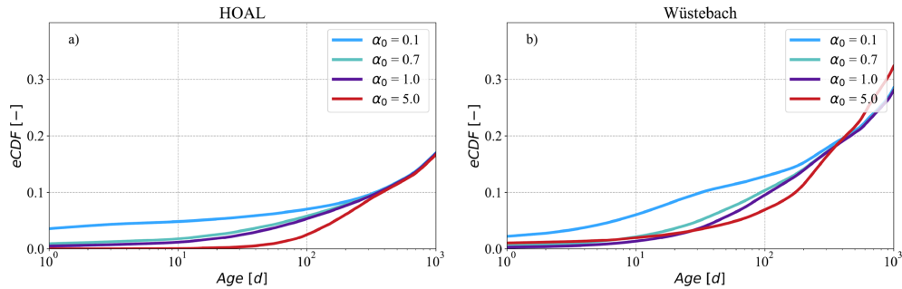
Figure 7. The mean of empirical cumulative distribution functions (eCDFs) of modelled transit times of daily discharge for the (a) HOAL and (b) Wüstebach catchments under varying SAS shape parameters in the unsaturated root zone ( \alpha_0 = 0.1, 0.7, 1.0, 5.0 ). (a, b) The simulations range from very young preference ( \alpha_0 = 0.1 ) to old water preference ( \alpha_0 = 5 ) for the unsaturated root zone preferential flow, while the groundwater flow was uniformly sampled ( \alpha = 1 ).
