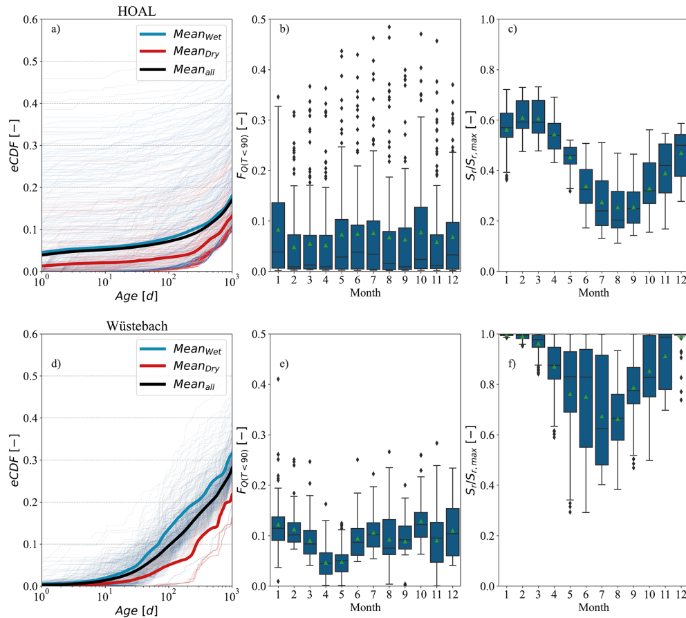
Figure 5. Modelled empirical cumulative transit time distributions (TTDs) for daily streamflow in the (a) HOAL and (d) Wüstebach catchments. The colour of the lines corresponds to the wetness state, where dark blue indicates a wet period and dark red indicates a dry period. In panels (a) and (d), the mean of the empirical cumulative TTDs is shown for the entire tracking period (black line), the dry period (red line), and the wet period (dark blue line). The fraction of streamflow younger than 90 d, F_Q(T < 90) , grouped by month of the year, is shown in panels (b) and (e) for the HOAL and Wüstebach catchments, respectively. modelled relative soil wetness ( \frac{S_r}{S_{r,max}} ), also grouped by month of the year, is shown in panels (c) and (f) for the HOAL and Wüstebach catchments, respectively. Green triangles in panels (b), (c), (e), and (f) show the mean values.
