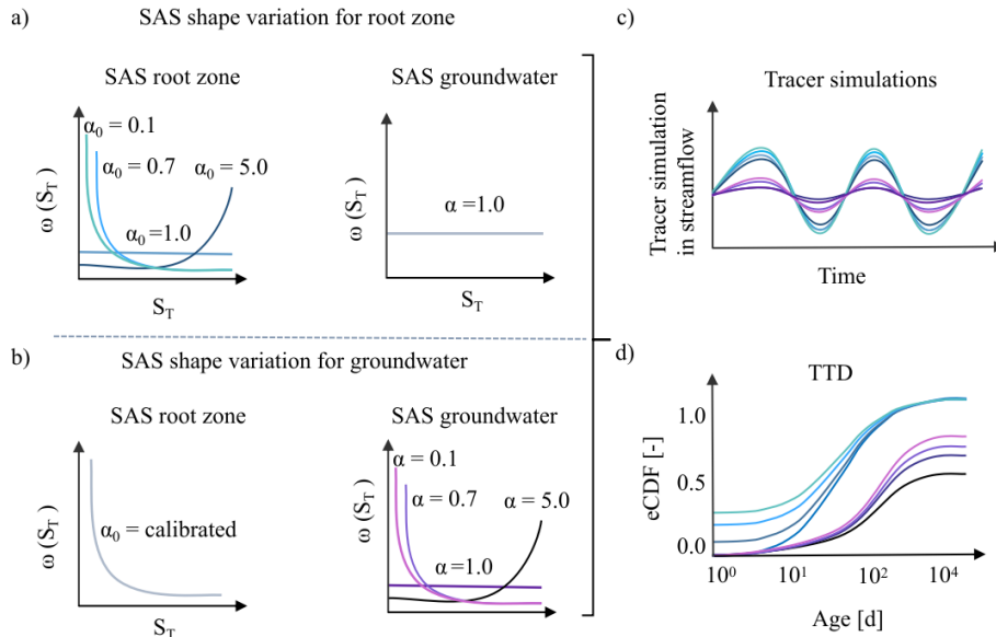
Figure 3. Conceptual representation of the sensitivity analysis illustrating how different SAS functions, formulated with the lower bound of the shape parameter \alpha_0 for root-zone preferential flow and \alpha for groundwater flow, affect the modelled tracer signals and inferred transit time distributions (TTDs). (a) The unsaturated root-zone SAS function shape parameter \alpha_0 is varied from 0.1 (strong young-water preference, light blue line) to 5.0 (old-water preference, dark blue line), while the groundwater age selection remains uniform. (b) The root-zone SAS function shape parameter \alpha_0 is fixed at its calibrated value, and the groundwater \alpha is varied from 0.1 (strong young-water preference, light purple line) to 5.0 (old-water preference, dark purple line). (a, b) The x-axis, S_T , represents the age-ranked storage, and the y-axis, \omega(S_T) , denotes the relative probability of releasing water of that age. (c, d) Illustrate the modelled tracer time series based on the scenarios implemented in (a) and (b), and the corresponding empirical cumulative transit time distributions.
