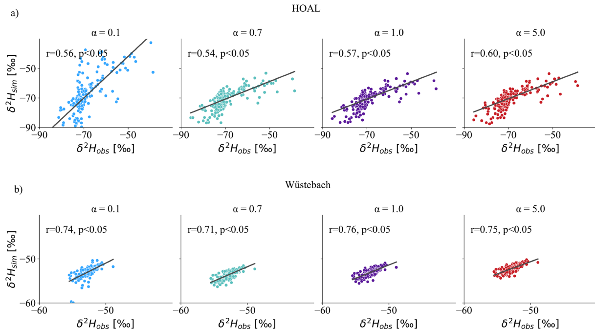
Figure 8. Spearman rank correlations between modelled ( y -axis) and observed ( x -axis) \delta^2\text{H} signals in streamflow based on varying the SAS shape parameter \alpha [–] in groundwater for (a) HOAL and (b) Wüstebach. The simulations ranged from very young water preference ( \alpha = 0.1 ) to old water preference ( \alpha = 5 ) for the groundwater, while for the root zone compartment, a calibrated value was used ( \alpha_0 = 0.14 for HOAL and 0.98 for Wüstebach).
