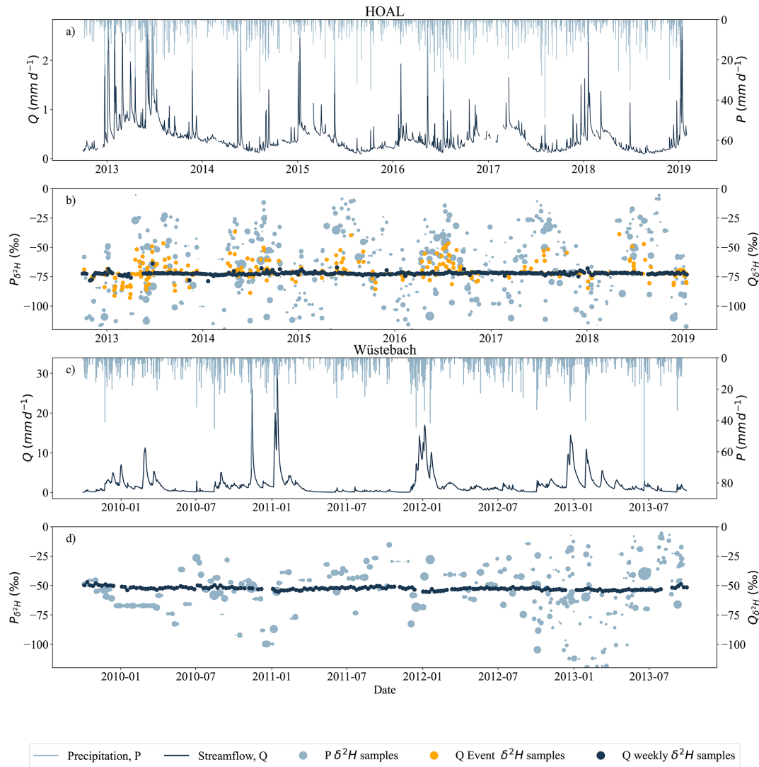
Figure 1. Hydrological and tracer data of the HOAL and Wüstabach catchments. (a, c) daily measured streamflow Q ( \text{mm d}^{-1} ) and precipitation P ( \text{mm d}^{-1} ). (b, d) precipitation \delta^2\text{H} signals (light blue) and streamflow \delta^2\text{H} signals (dark blue); the size of the dots indicates the relative precipitation volume. For the HOAL catchment, the \delta^2\text{H} data of streamflow were further shown as the weekly grab samples (b, dark blue dots) and event samples (b, orange dots). For the HOAL catchment, precipitation \delta^2\text{H} samples are in daily resolution, whereas for the Wüstabach catchment, beginning in September 2012, the sampling frequency for precipitation \delta^2\text{H} increased from weekly to daily (d).
