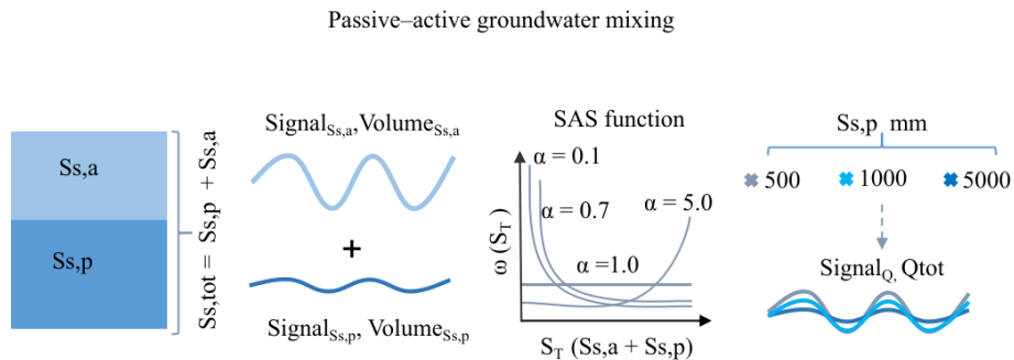
Figure 4. Conceptual representation of the sensitivity analysis illustrating how different passive storage volumes ( S_{s,p} = 500, 1000, and 5000 mm) interact with the active storage volume ( S_{s,a} ) under various groundwater SAS function shapes affecting tracer simulations in streamflow. The groundwater SAS function parameter \alpha is varied from 0.1 (strong young-water preference) to 5.0 (old-water preference). For the SAS function, the x-axis, S_T , represents the age-ranked total groundwater storage, and the y-axis, \omega(S_T) , denotes the relative probability of releasing water of that age.
