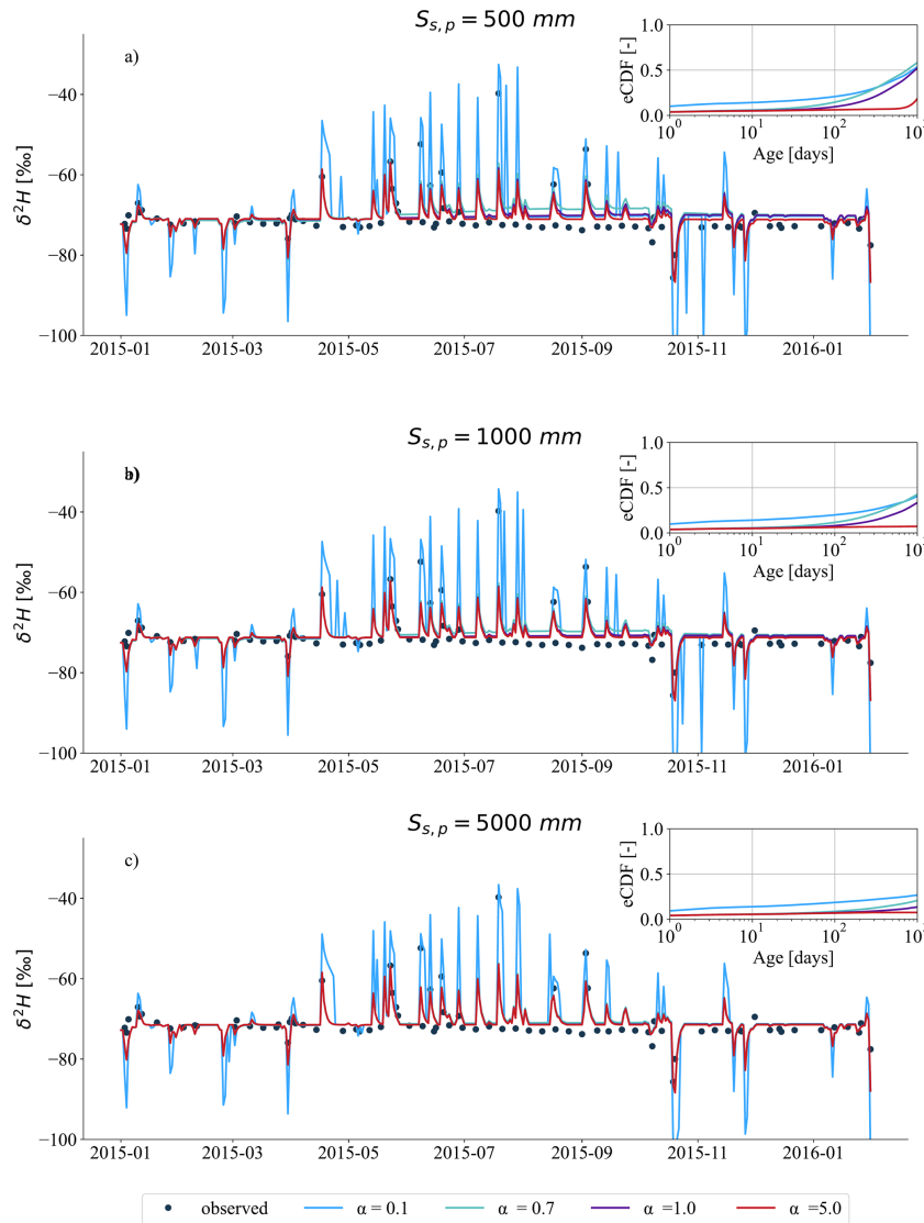
Figure 11. modelled \delta^2\text{H} signals in streamflow ( Q ; \text{mm d}^{-1} ) for the HOAL catchment in the year 2015, based on varying passive groundwater storage volumes ( S_{s,p} = 500, 1000, \text{ and } 5000 \text{ mm} ) and different mixing assumptions defined by SAS function shape parameters ( \alpha = 0.1, 0.7, 1.0, \text{ and } 5.0 ). (a–c) Each plot shows results for one S_{s,p} value, with black dots indicating observed grab samples of streamflow \delta^2\text{H} , and coloured lines representing modelled \delta^2\text{H} under the different \alpha values. The inset in each plot shows the mean empirical cumulative distribution functions (CDF) of modelled daily streamflow transit times during the tracking period (2015–2019); line colours correspond to \alpha values: blue for 0.1, turquoise for 0.7, purple for 1.0, and red for 5.0. Simulations over the full tracking period (2015–2019) are provided in the Fig. S11.
