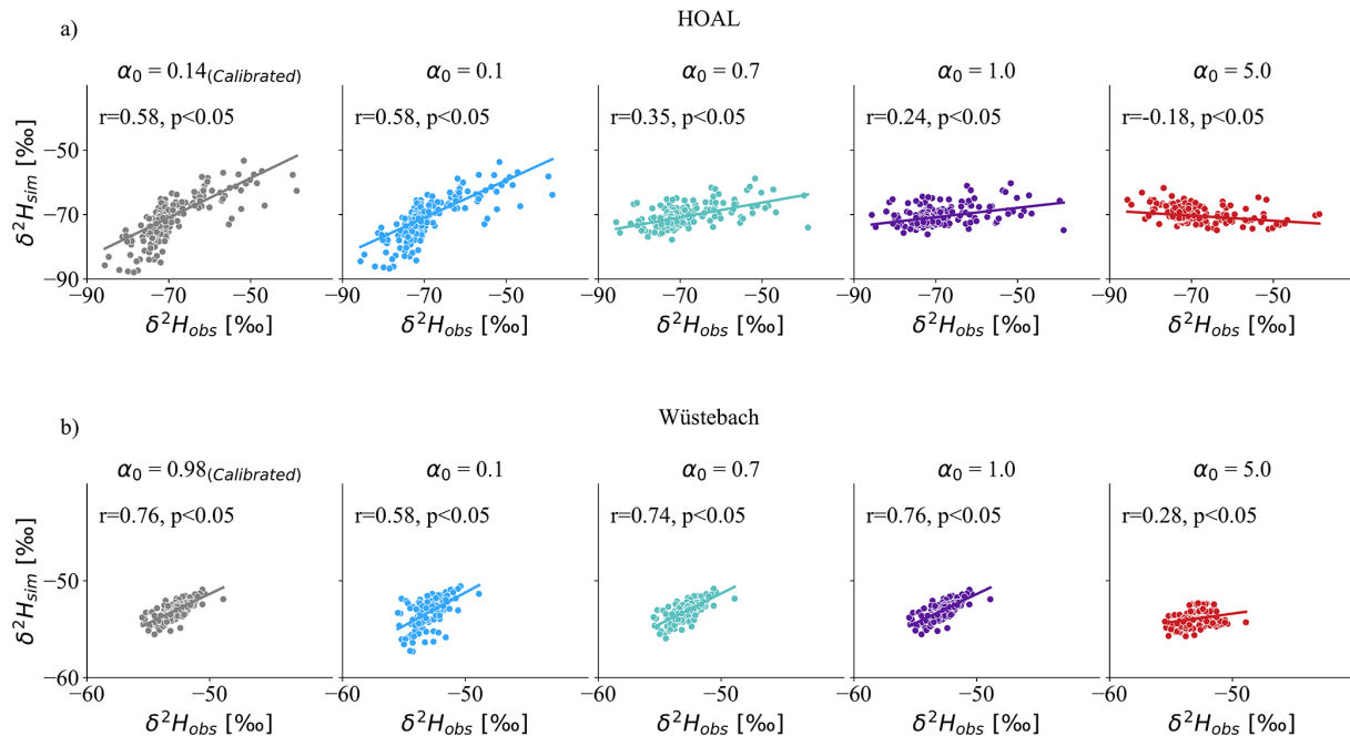
Figure 6. Spearman rank correlations between modelled (y-axis) and observed (x-axis) \delta^2H signals in streamflow based on varying the SAS shape parameter \alpha_0 [–] in the root zone for (a) HOAL and (b) Wüstebach. The simulations range from very young preference ( \alpha_0 = 0.1 ) to old water preference ( \alpha_0 = 5 ) for the unsaturated root zone preferential flow, while the groundwater flow was uniformly sampled ( \alpha = 1 ).
