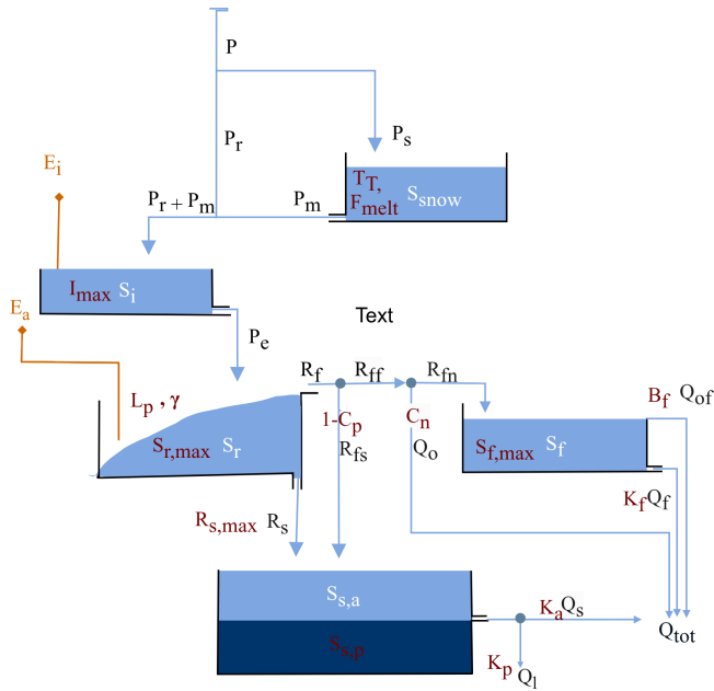
Figure 2. The model structure used to represent the HOAL and the Wüstebach catchment (adapted from Türk et al., 2025). Light blue boxes indicate the hydrologically active storage volumes that contribute to total discharge Q_{tot} : Snow storage ( S_{snow} ), canopy interception ( S_i ), fast response bucket ( S_f ), root zone storage ( S_r ), and “active” groundwater ( S_{s,a} ). The darker blue box ( S_{s,p} ) indicates a hydrologically “passive” groundwater volume. Blue lines indicate snow and water fluxes which are total precipitation P ( \text{mm d}^{-1} ), precipitation as snow P_s ( \text{mm d}^{-1} ), precipitation as rain P_r ( \text{mm d}^{-1} ), snow-melt P_m ( \text{mm d}^{-1} ), throughfall P_e ( \text{mm d}^{-1} ), preferential fast response R_f ( \text{mm d}^{-1} ), fast preferential recharge to the to groundwater R_{fs} ( \text{mm d}^{-1} ), preferential fast response R_{ff} ( \text{mm d}^{-1} ), infiltration-excess overland flow Q_o ( \text{mm d}^{-1} ), preferential fast response to the fast-responder R_{fn} ( \text{mm d}^{-1} ), flow from the fast-responder Q_f ( \text{mm d}^{-1} ), saturation-excess overland flow from the fast-response bucket Q_{of} ( \text{mm d}^{-1} ), slow recharge to the groundwater reservoir R_s ( \text{mm d}^{-1} ), baseflow from the groundwater reservoir Q_s ( \text{mm d}^{-1} ), deep infiltration loss Q_l ( \text{mm d}^{-1} ), and the total discharge to the streamflow Q_{tot} ( \text{mm d}^{-1} ). Orange lines indicate water vapour fluxes; interception evaporation E_i ( \text{mm d}^{-1} ), evaporation from the root zone E_a ( \text{mm d}^{-1} ). Model parameters are shown in red adjacent to the model component they are associated with, and symbols are defined in Table S2. All model equations are defined in Table S1.
