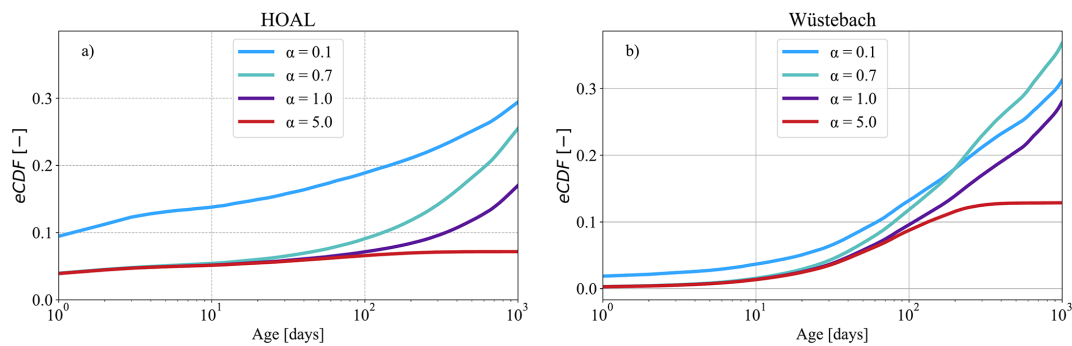
Figure 10. The mean of empirical cumulative distribution functions (eCDFs) of modelled transit times of daily discharge for the (a) HOAL and (b) Wüstebach catchments under varying SAS shape parameters ( \alpha = 0.1, 0.7, 1.0, 5.0 ) for groundwater. Lower \alpha values favour younger water, producing younger transit time distributions, while higher \alpha values shift the distribution toward older water. The mean of inferred TTD lines are illustrated with blue, turquoise, purple, and red lines corresponding to \alpha values of 0.1, 0.7, 1.0, and 5.0, respectively. The simulations ranged from very young water preference ( \alpha = 0.1 ) to old water preference ( \alpha = 5 ) for the groundwater, while for the root zone compartment, a calibrated value was used ( \alpha_0 = 0.14 , for HOAL and 0.98 for Wüstebach).
