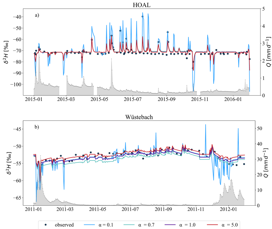
Figure 9. Simulation of \delta^2\text{H} in streamflow based on varying SAS shape parameter \alpha [–] in groundwater for (a) HOAL shown for 2015 and (b) Wüstebach shown for 2011. Simulations over the full tracking period are provided in Fig. S9. The simulations ranged from very young water preference ( \alpha = 0.1 ) to old water preference ( \alpha = 5 ) for the groundwater, while for the root zone compartment, a calibrated value was used ( \alpha_0 = 0.14 , for HOAL and 0.98 for Wüstebach). The modelled \delta^2\text{H} signals from the model are illustrated with blue, turquoise, purple, and red lines corresponding to \alpha values of 0.1, 0.7, 1.0, and 5.0, respectively. The grey-shaded area shows the measured streamflow ( Q , \text{mm d}^{-1} ) for both catchments.
