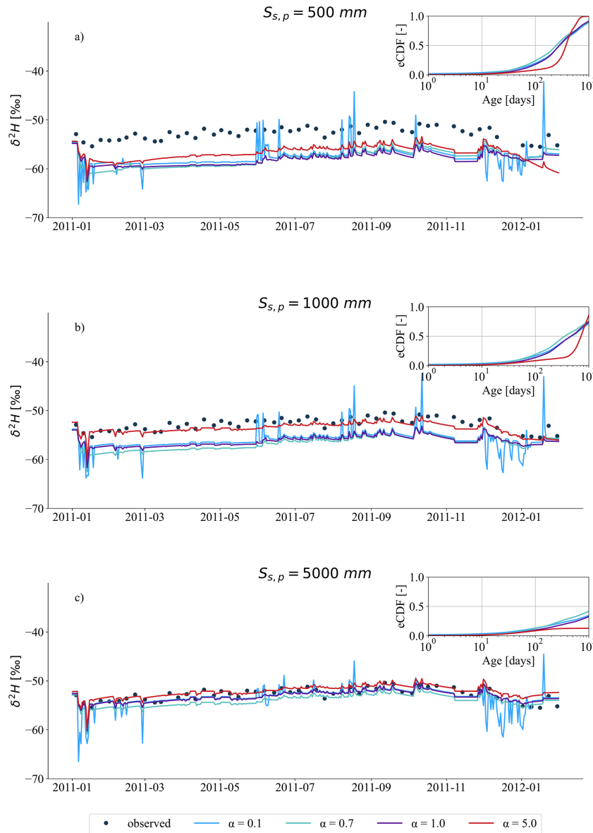
Figure 12. Modelled \delta^2\text{H} signals in streamflow ( Q , \text{mm d}^{-1} ) for the Wüstabach catchment in the year 2011, based on varying passive groundwater storage volumes ( S_{S,p} = 500, 1000, \text{ and } 5000 \text{ mm} ) and different mixing assumptions defined by SAS function shape parameters ( \alpha = 0.1, 0.7, 1.0, \text{ and } 5.0 ). (a–c) Each plot shows results for one S_{S,p} value, with black dots indicating observed grab samples of streamflow \delta^2\text{H} , and coloured lines representing modelled \delta^2\text{H} under the different \alpha values. The inset in each plot shows the mean empirical cumulative distribution functions (eCDFs) of modelled daily streamflow transit times during the tracking period. Line colours correspond to \alpha values: blue for 0.1, turquoise for 0.7, purple for 1.0, and red for 5.0. Simulations over the full tracking period (2011–2013) are provided in the Fig. S12.
