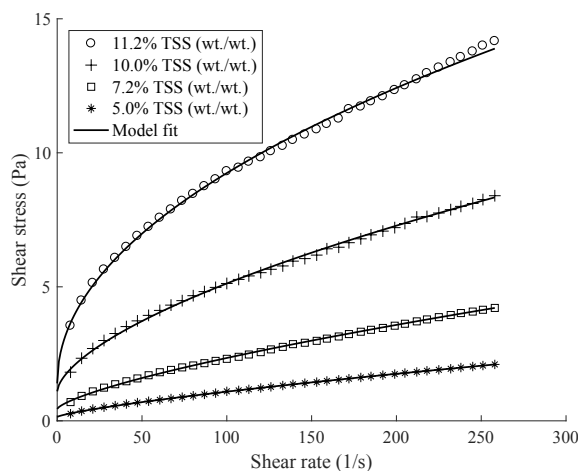
Figure 2.7: Rheogram of slurry 1 at various concentration and a fixed temperature of 20°C; the respective model used for fitting is indicated in table 2.
