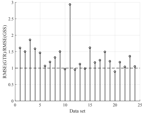
Figure 2.11: Plotting the ratio of the RMSE from the algorithm GTR to the one from GSS of the for the data set of Slurry 1 concentration ranging 11.2 till 3.2 % TSS of temperatures 10^\circ C , 20^\circ C , 30^\circ C , 40^\circ C .
