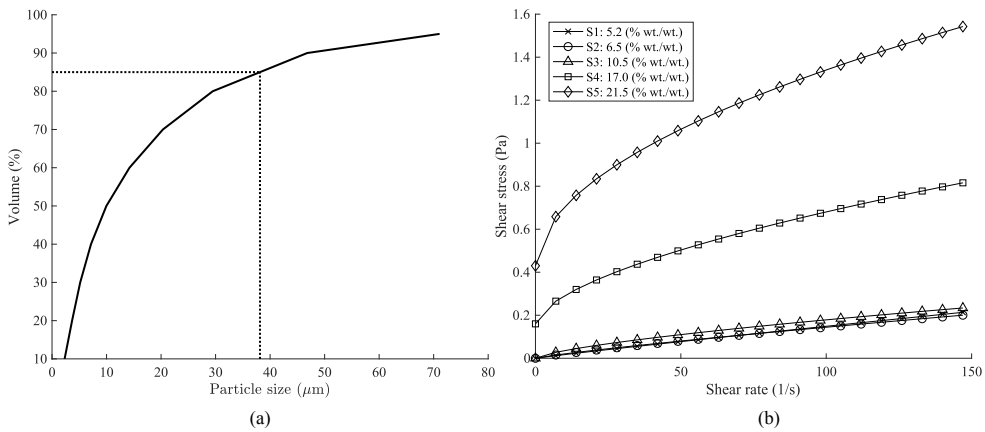
Figure 4.3: Cumulative particle size distribution of suspended slurry particulates in water with a D_{85} of 38\mu\text{m} .
