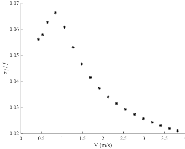
Figure 4.4: Uncertainty in the friction factor
