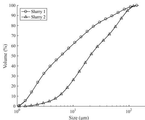
Figure 2.2: Cumulative particle size distribution of slurry 1 and slurry 2.
