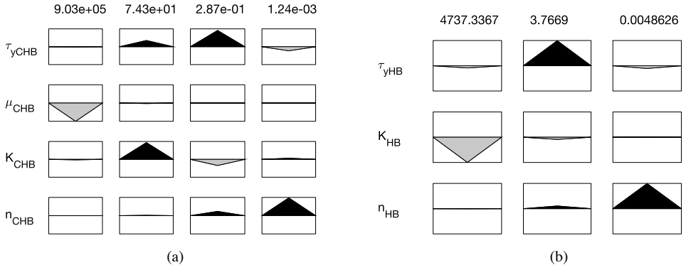
Figure 2.10: Singular values and eigen vectors of the parameters for (a) CHB model and (b) HB model using rheometric data of slurry 1 at 20^\circ C with 11.2 % TSS.
