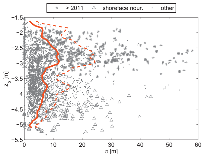
Fig. 13. Comparison of sand bar variability (horizontal axis) and bar crest depth (vertical axis). Data points obtained around the end points of shoreface nourishments have been marked with triangles, while data points obtained after 2011 have been marked with stars. The solid line represents a window-averaged variability in a sliding depth window of 0.25 m (excluding shoreface nourishment data points). The windowed average plus one windowed standard deviation is indicated with a dashed line.
