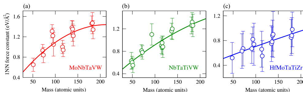
Fig. 5 Absolute values of the x-x components of the nearest-neighbor force constants of the respective 15 elemental pairs in the 5-component alloys a MoNbTaVW, b NbTaTiVW, and c HfMoTaTiZr. The force constants are shown versus the square-root of the mass product of the atomic pairs including the standard deviation as obtained from the force constant distributions shown in Fig. 4c. The lines are second order polynomial fits to the data. The atomic mass correlates with the computed force constants: the larger the mass, the larger the force constants. This correlation causes a partial compensation of the mass fluctuation induced phonon broadening by the force constant fluctuations
