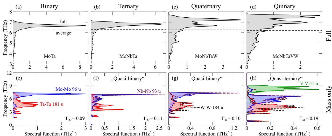
Fig. 2 a–d : Full spectral functions of the first alloy series (MoTa to MoNbTaVW) at the H-point. The dashed lines represent the spectral function (delta peaks) employing averaged force constants and masses. e–h : Spectral functions at the H-point projected on elemental pairs (Mo-Mo blue solid lines with blue shading, Ta-Ta red solid lines with red shading, Nb-Nb dark violet dashed lines, W-W black dashed lines, and V-V green solid lines with green shading) including only mass fluctuations (averaged force constants)
