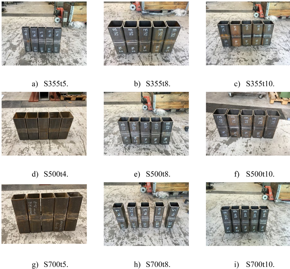
Fig. 1. Welded tubes.
