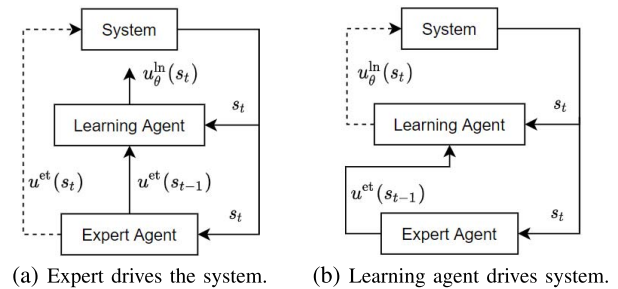
Fig. 1. Learning settings.
