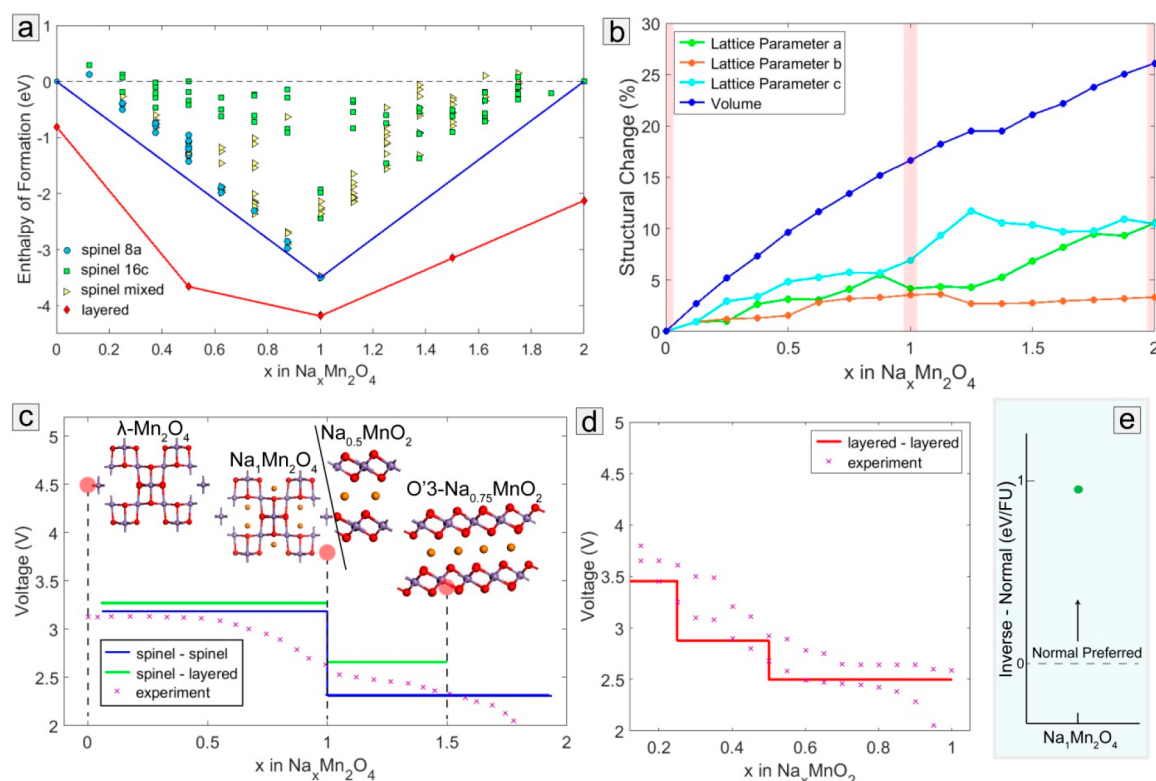
Figure 4. (a) Enthalpies of formation and convex hull of Na insertion in \lambda - \text{Mn}_2\text{O}_4 and layered O3 \text{MnO}_2 . Cyan circles, green squares, and yellow triangles represent Na inserting into only 8a, only 16c, and mixed spinel interstitial sites, respectively. Red diamonds represent Na intercalation in the O3 layered structure. Blue and red lines follow the lowest enthalpy path of the spinel and layered structure, respectively. (b) Structural changes during Na insertion in \lambda - \text{Mn}_2\text{O}_4 ; the light red vertical lines indicate the stable phases during the sodiation process. (c) Calculated (blue line) vs experimental 10,15 (scatter) voltage profile of Na insertion in \lambda - \text{Mn}_2\text{O}_4 . The experimental data were normalized according to what is considered as full capacity reaching the \text{Na}_1\text{Mn}_2\text{O}_4 and \text{Na}_1\text{Mn}_{1.5}\text{Ni}_{0.25}\text{O}_4 phase. 10,15 The green lines indicate the average voltages between the spinel and the layered O'3- \text{Na}_{0.5}\text{MnO}_2 and O'3- \text{Na}_{0.75}\text{MnO}_2 monoclinic phases (please note the different stoichiometric notation). (d) Calculated (red line) vs experimental 54 (scatter) voltage profile of Na intercalation in the layered O3 structure. (e) The relative stability of the normal vs inverse spinel for the \text{Na}_1\text{Mn}_2\text{O}_4 concentration, where FU is the \text{Na}_1\text{Mn}_2\text{O}_4 formula unit.
