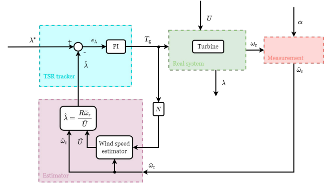
Fig. 1. Block diagram of the combined wind speed estimator and tip-speed ratio tracking control scheme. The green box represents the NREL's 5MW reference wind turbine. The wind speed estimator is indicated in purple, and the tip-speed ratio tracker is indicated in cyan. A sensor fault occurs at the rotor speed measurement in red.
