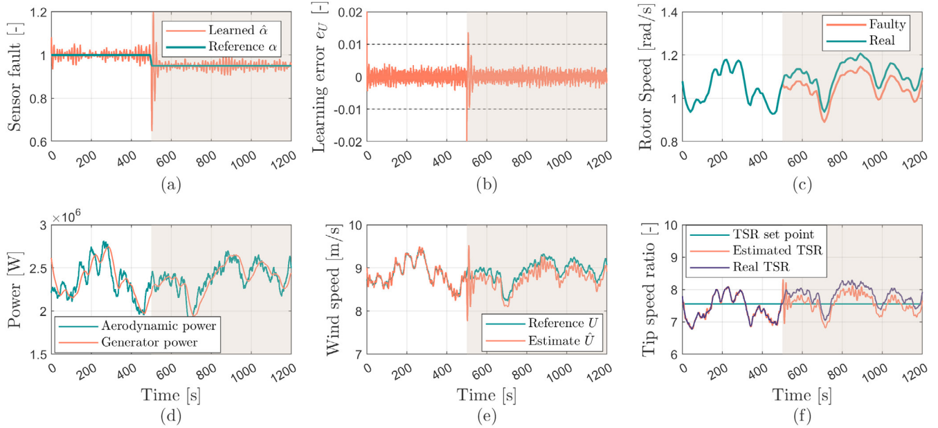
Fig. 3. Case study of the FTC method where only the fault detection and estimation step is activated. A turbulent wind condition with a mean wind speed of 9 m/s and TI of 5 % is considered. The iterative learning method is implemented online. The sensor fault occurs between 500 s and 1200 s as indicated by the olive background.
