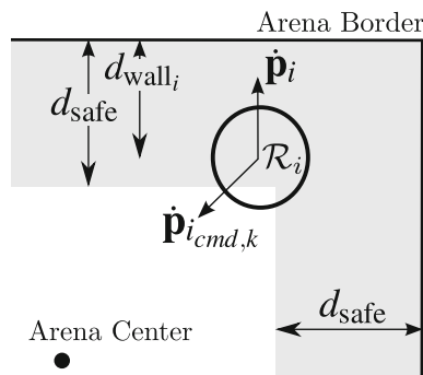
Fig. 8 Depiction of condition M1. Robot \mathcal{R}_i is too close to the border of the arena and receives a command to go towards the center
