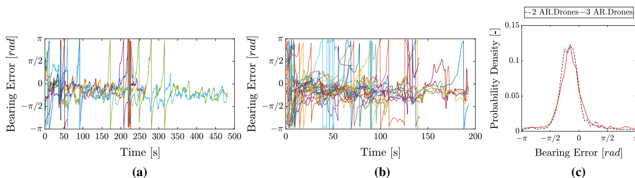
Fig. 19 Overview of relative bearing estimation errors for flights with two AR.Drones and three AR.Drones featuring on-board own-state estimation. a With two AR.Drones, b with three AR.Drones, c bearing error distribution for all flights
