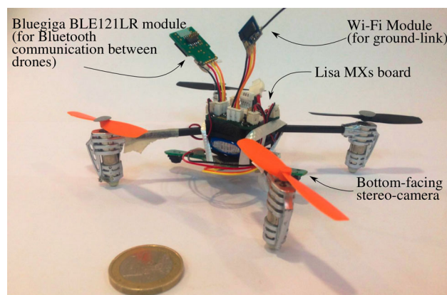
Fig. 20 Miniature drone used in the experiments
