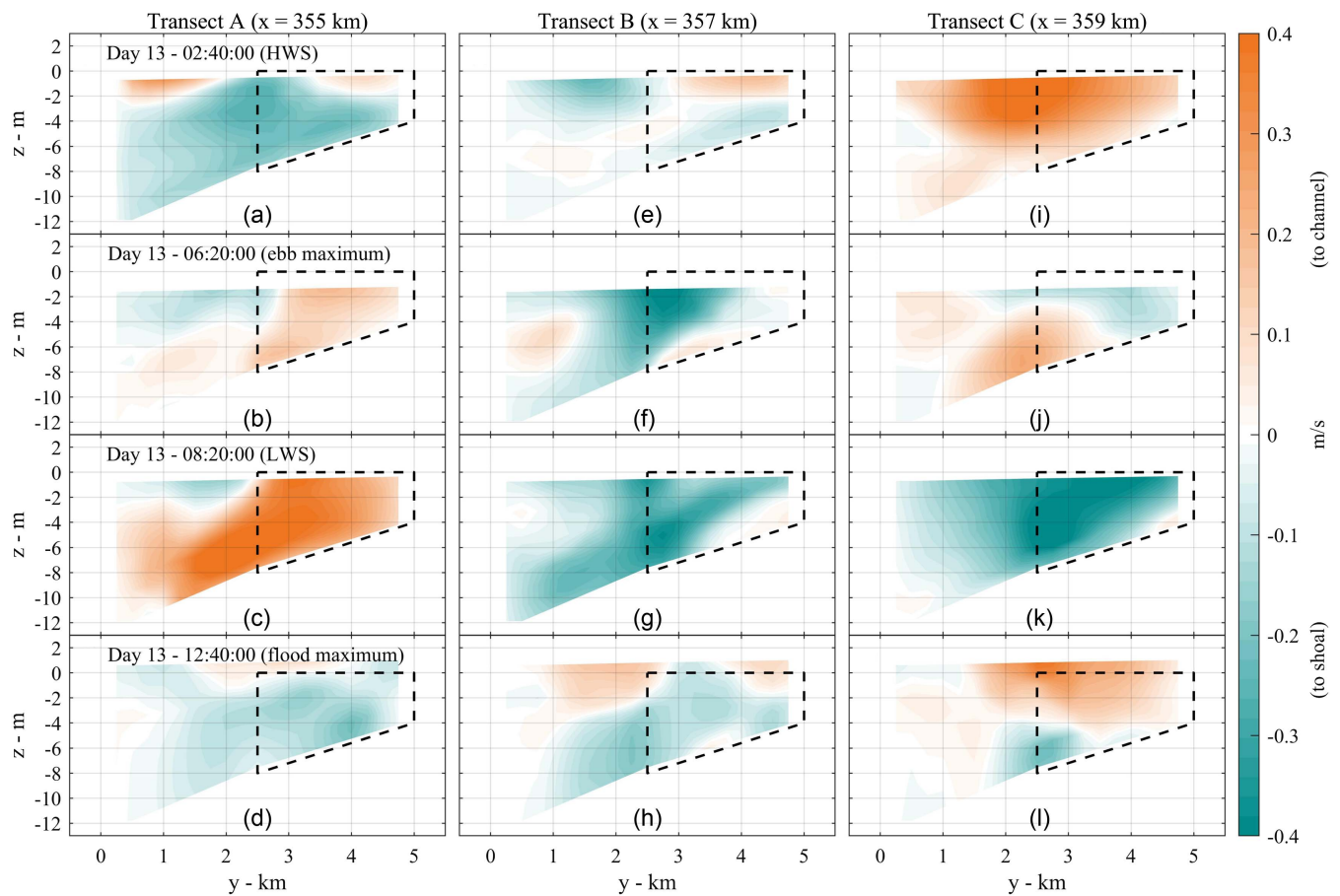
Fig. 5. Lateral flows on three cross-channel transects in Case 0: (a–d) Transect A at x = 355 km (1 km downstream to a groyne); (a) Day 13 - 02:40:00 (HWS); (b) Day 13 - 06:20:00 (ebb maximum); (c) Day 13 - 08:20:00 (LWS); and (d) Day 13 - 12:40:00 (flood maximum); (e–h) Transect B at x = 357 km (at the middle of a groyne field); and (i–l) Transect C at x = 359 km (1 km upstream to a groyne) at (a, e, and i) HWS; (b, f, and j) ebb maximum; (c, g, and k) LWS; and (d, h, and l) flood maximum. The four time periods are identical with those in Fig. 4. Dashed lines indicate position of groynes.
