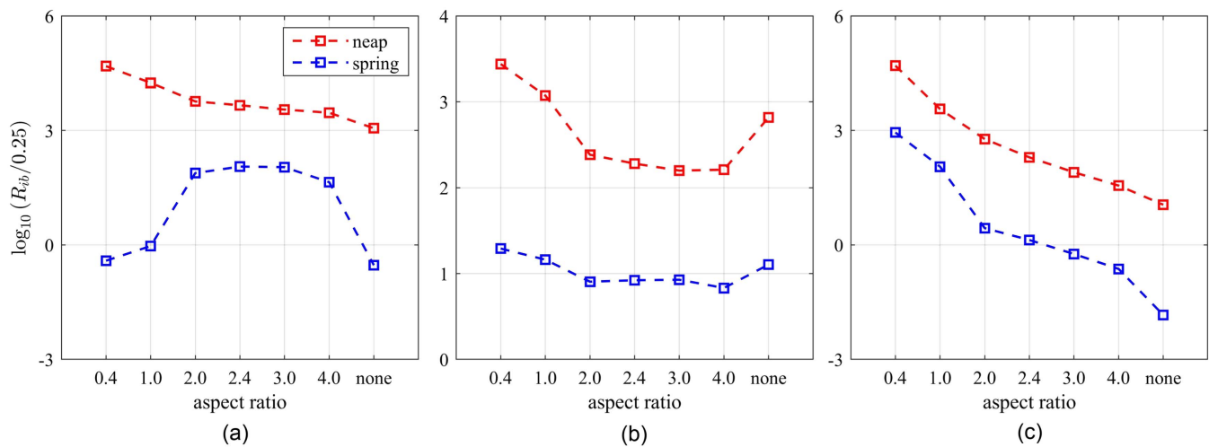
Fig. 14. Spatially averaged \log_{10}(R_{ib}/0.25) in (a) river; (b) main channel; and (c) groyne field.
