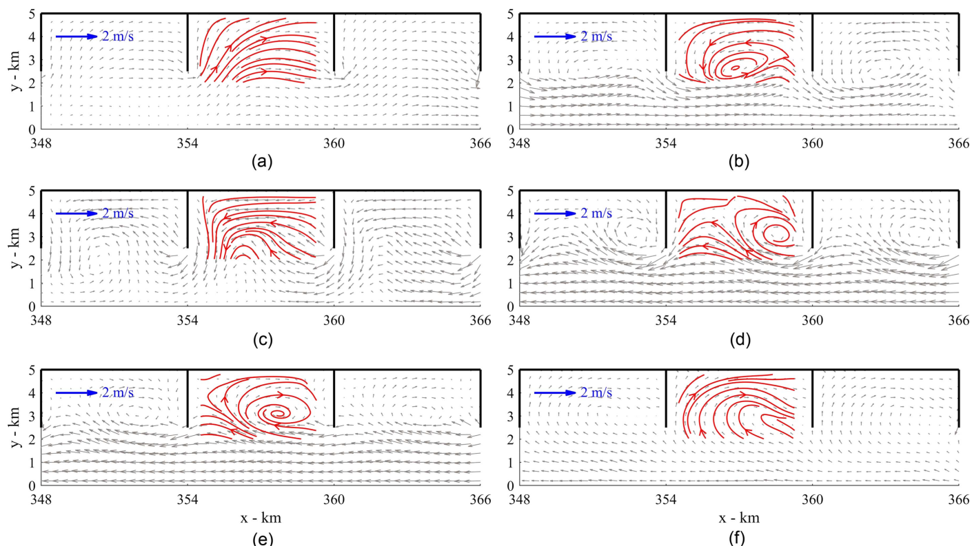
Fig. 7. Velocity vectors (gray arrows) in the main channel and streamlines (lines) in the groyne field during moderate tides at (a) 02:40:00 (high-water slack); (b) 07:00:00; (c) 08:20:00 (low-water slack); (d) 11:00:00; (e) 12:00:00; and (f) 14:40:00 in Day 13. Other arrows are length scales for velocity vectors. Velocity data are from the bottom layer of Case 0.
