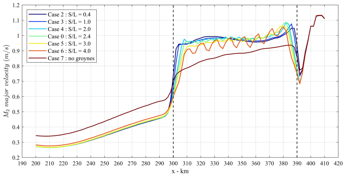
Fig. 8. Longitudinal distribution of major velocity of M_2 tide in scenarios with different numbers of groynes, by harmonic analysis for depth-averaged longitudinal velocity. Dashed lines indicate the upstream and downstream boundaries of the channel.
