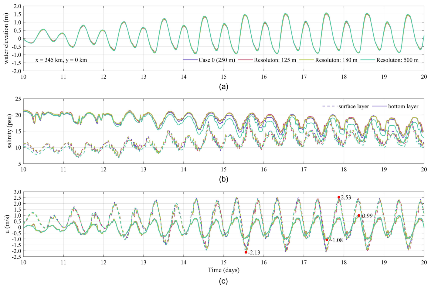
Fig. 2. (a) Water elevations; (b) surface and bottom salinity; and (c) surface and bottom flow velocity at the middle of the main channel ( x = 345 km, y = 0 km) in Case 0 with four grid resolutions. Typical velocities are marked in panel (c).
