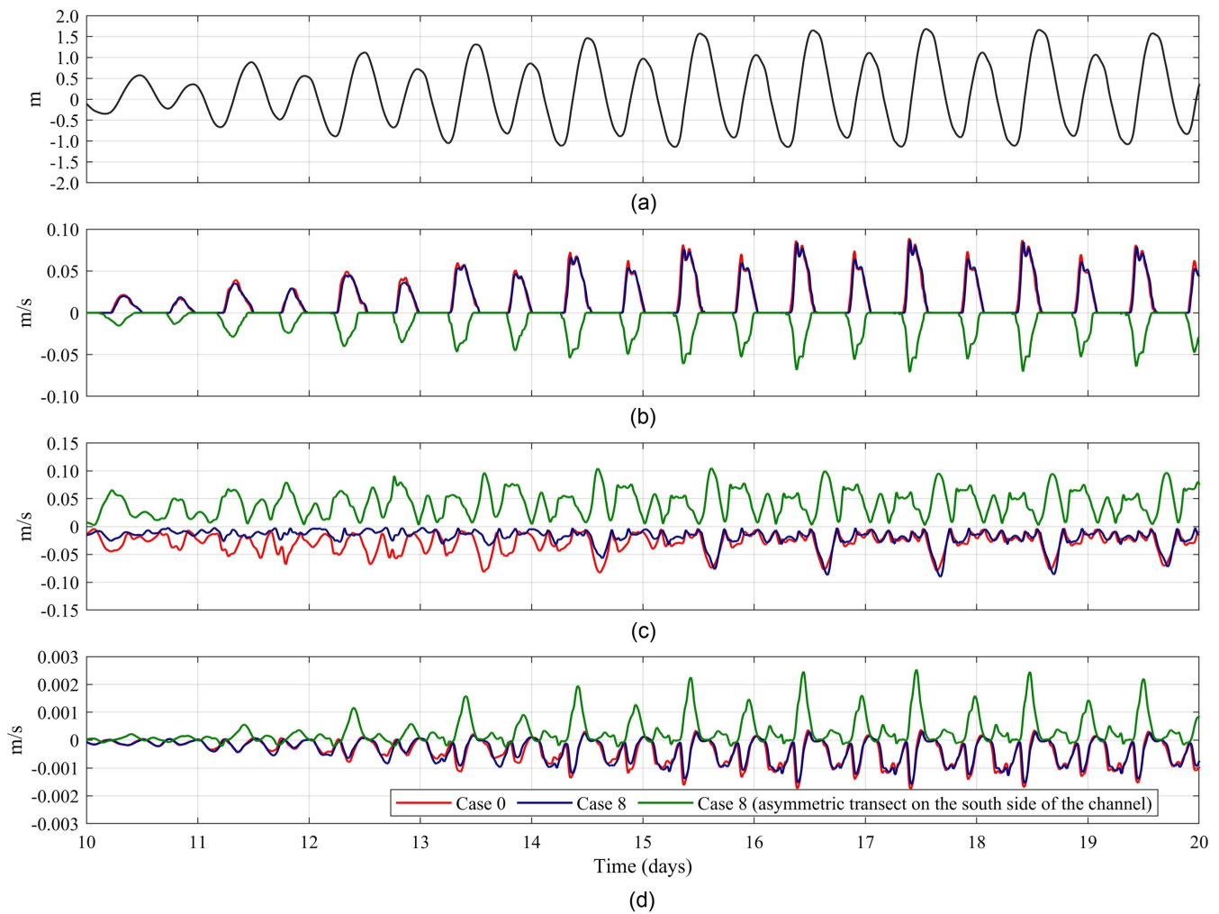
Fig. 10. (a) Water level in Case 0 averaged on an along-channel transect [Transect D in Fig. 4(a)]; (b) tidal filling component of exchange velocity, inflowing from the main channel to groyne fields ( v_{\text{tidal,in}} ); (c) vertical component of exchange velocity outflowing from groyne fields to the main channel ( v_{\text{ver,out}} ); and (d) net vertical component of exchange velocity (net v_{\text{ver}} ).
