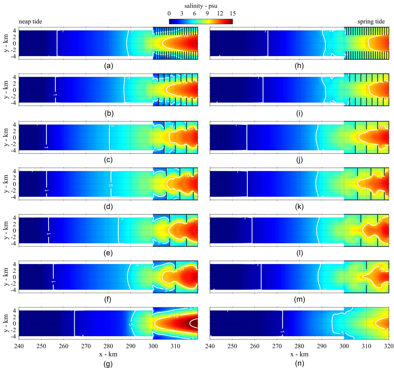
Fig. 11. Saltwater intrusion in different scenarios during neap tide and spring tide. Contour lines of 1, 5, 10, and 15 psu in the bottom layer are shown with open lines: (a) Case 2, time = 11 03:00:00, S/L = 0.4 ; (b) Case 3, time = 11 03:00:00, S/L = 1 ; (c) Case 4, time = 11 03:00:00, S/L = 2 ; (d) Case 0, time = 11 03:00:00, S/L = 2.4 ; (e) Case 5, time = 11 03:00:00, S/L = 3 ; (f) Case 6, time = 11 03:00:00, S/L = 4 ; (g) Case 7, time = 11 03:00:00; (h) Case 2, time = 15 04:30:00, S/L = 0.4 ; (i) Case 3, time = 15 04:30:00, S/L = 1 ; (j) Case 4, time = 15 04:30:00, S/L = 2 ; (k) Case 0, time = 15 04:30:00, S/L = 2.4 ; (l) Case 5, time = 15 04:30:00, S/L = 3 ; (m) Case 6, time = 15 04:30:00, S/L = 4 ; and (n) Case 7, time = 15 04:30:00.
