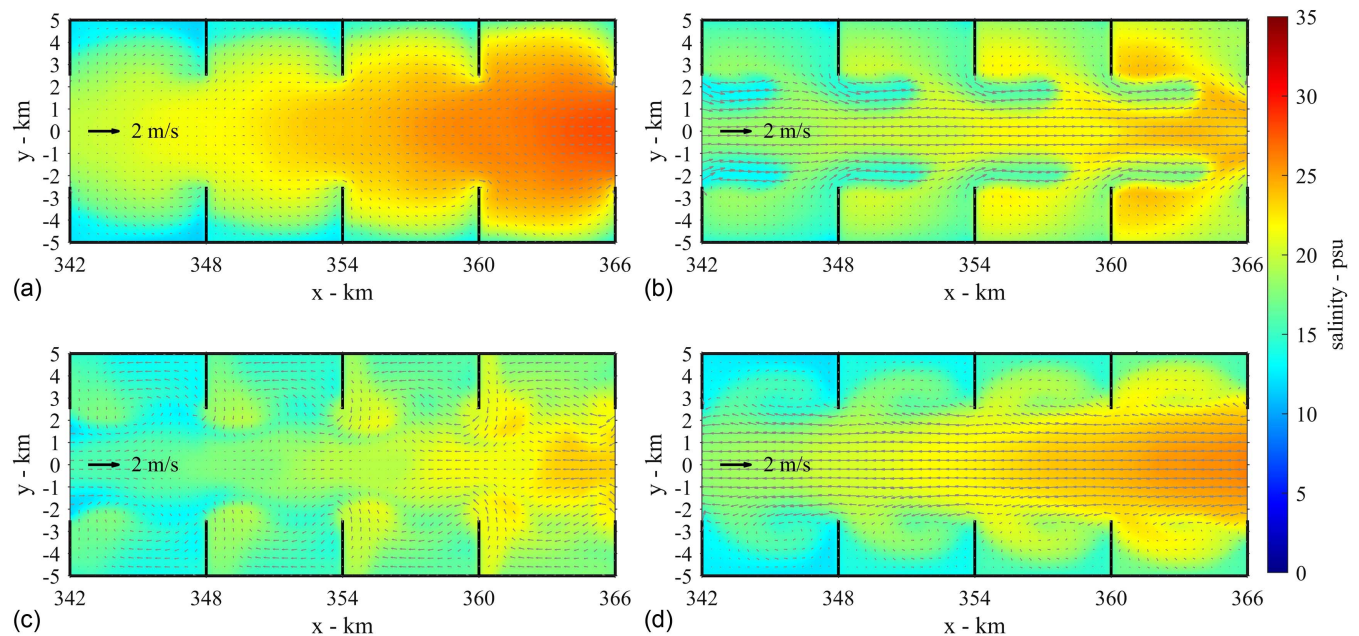
Fig. 6. Bottom salinity distribution in Case 0 at four moments corresponding to time periods in Fig. 4: (a) HWS (Day 13 - 02:40:00); (b) peak ebb (Day 13 - 06:20:00); (c) LWS (Day 13 - 08:20:00); and (d) peak flood (Day 13 - 12:40:00).
