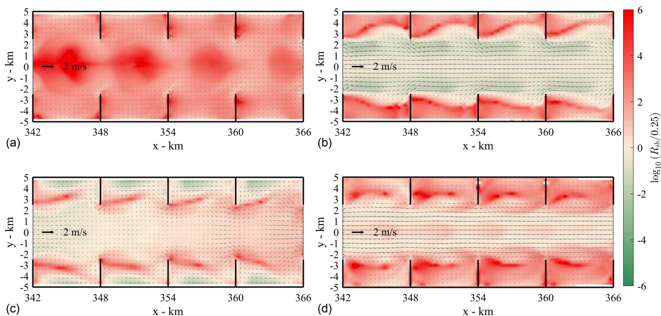
Fig. 3. Distribution of bulk Richardson number [\log_{10}(R_{ib}/0.25)] and velocity vectors in the channel for (a) high-water slack [Case 0, Day 13 - 02:40:00 (HWS)]; (b) peak ebb currents [Case 0, Day 13 - 06:20:00 (peak ebb)]; (c) low-water slack [Case 0, Day 13 - 08:20:00 (LWS)]; and (d) peak flood currents [Case 0, Day 13 - 12:40:00 (peak flood)]. High-water slack and low-water slack conditions are based on flow velocity reversal. Results are from Case 0.
