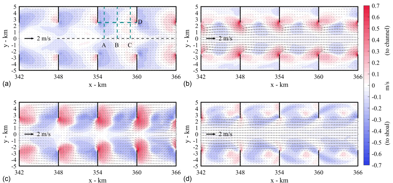
Fig. 4. Bottom lateral current velocities and velocity vectors at (a) HWS [Case 0, Day 13 - 02:40:00 (HWS)]; (b) ebb maximum [Case 0, Day 13 - 06:20:00 (peak ebb)]; (c) LWS [Case 0, Day 13 - 08:20:00 (LWS)]; and (d) flood maximum [Case 0, Day 13 - 12:40:00 (peak flood)]. A positive value indicates a direction from groyne fields to the main channel (STC, from both sides). These results are from Case 0 in moderate tidal conditions. Three cross-channel and one along-channel transects are marked with dashed lines.
