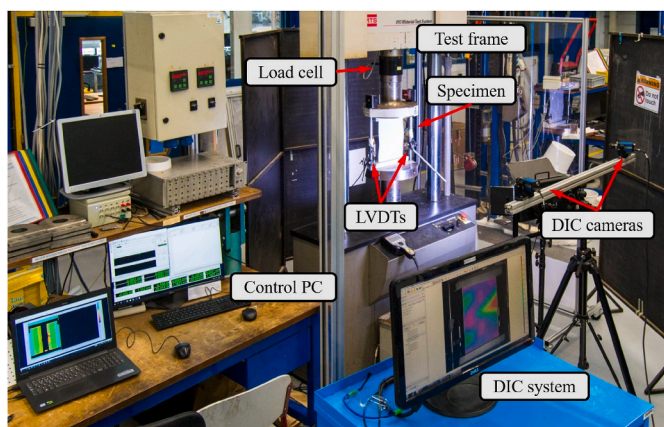
Fig. 3. Test set-up.
