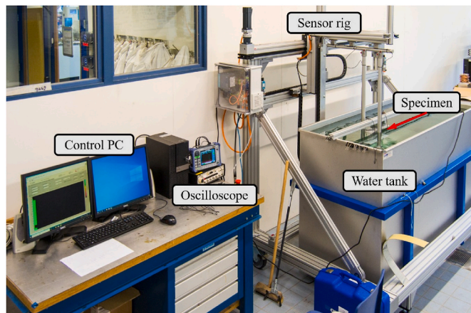
Fig. 4. Ultrasonic C-scan system.
