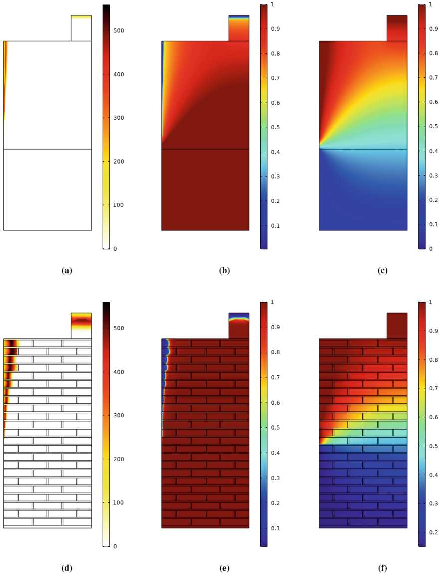
Fig. 5. Distribution maps of c_s^s , S_w^l and \omega/\omega_{\text{sat}} respectively for the homogeneous model (a, b, c) and the textured model (d, e, f).
