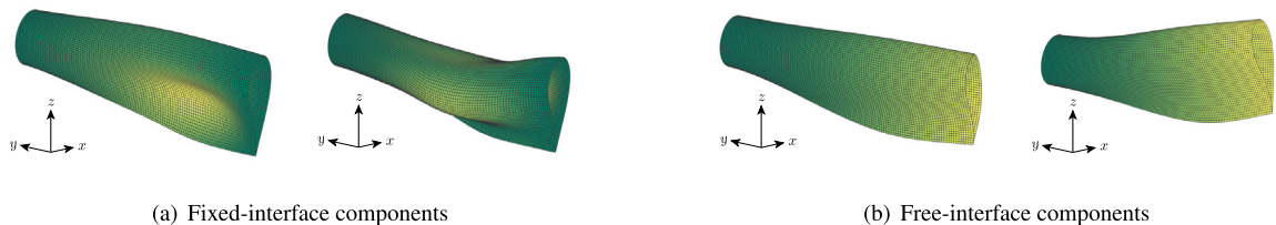
Fig. 12. The first two fixed- and free-interface components of the blade substructure.
