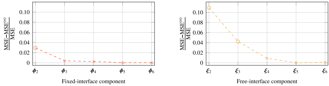
Fig. 8. Selection of basis vectors for fixed- (left) and free-interface methods (right).
