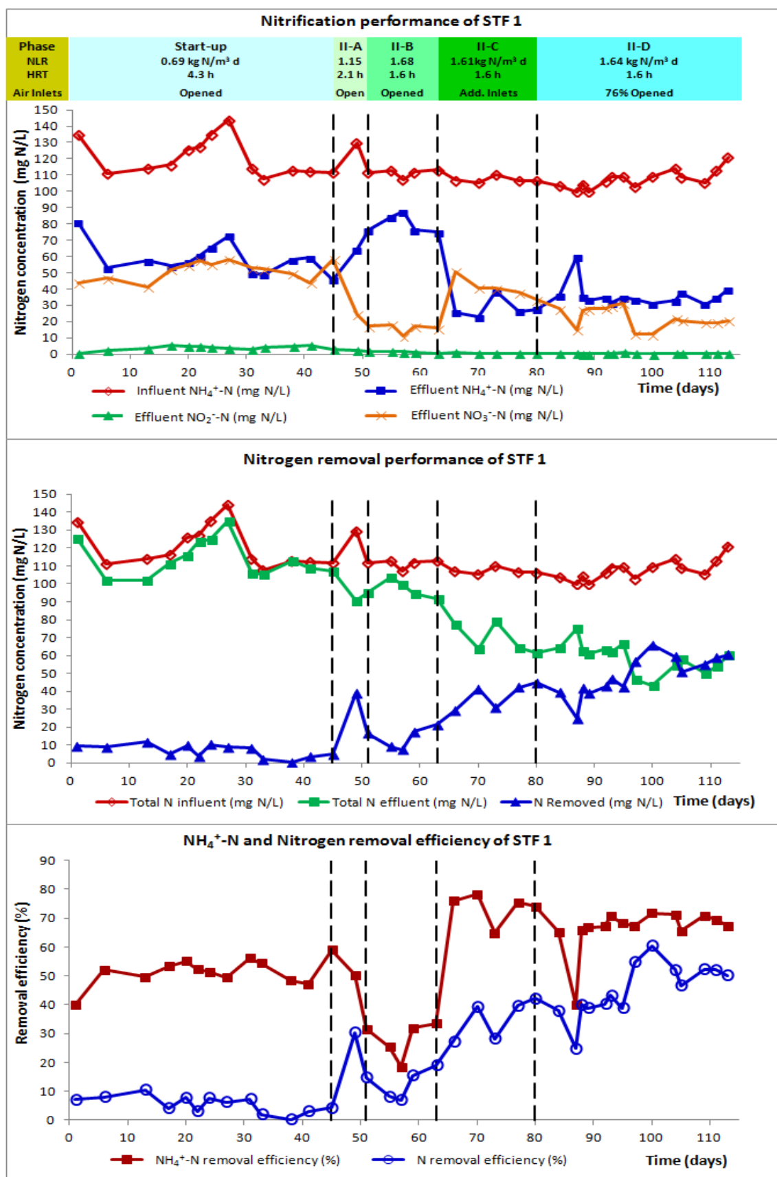
Figure 5.3. \text{NH}_4^+\text{-N} removal performance of STF-1.
