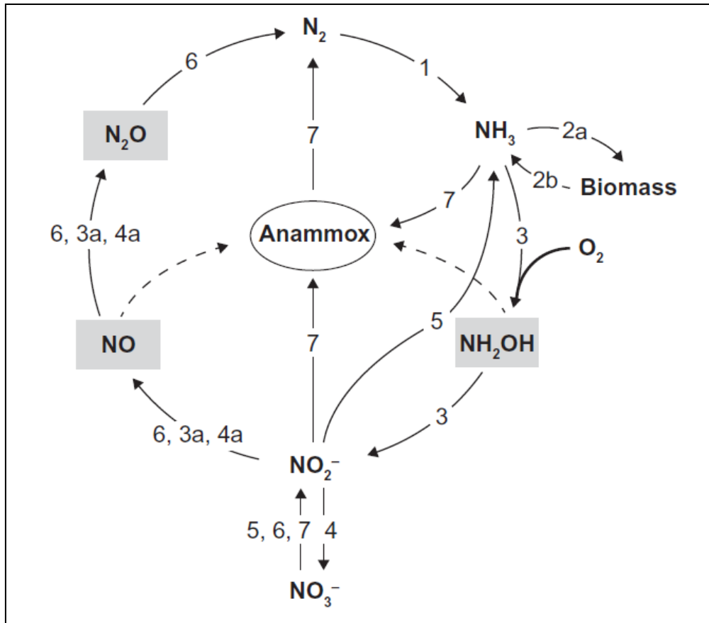
Figure 1.3. The nitrogen cycle: depicting the position of Anammox bacteria and partial oxidation and reduction processes: (1) nitrogen fixation; (2a) ammonium assimilation; (2b) ammonification/mineralization; (3) aerobic ammonium oxidation; (4) nitrite oxidation; (3a) and (4a) anaerobic nitrification-denitrification by ammonium and nitrite oxidizing nitrifiers, respectively; (5) dissimilatory nitrite reduction to ammonium (DNRA); (6) anaerobic denitrification; (7) anammox (Source: adapted from Kartal et al. , 2012).
