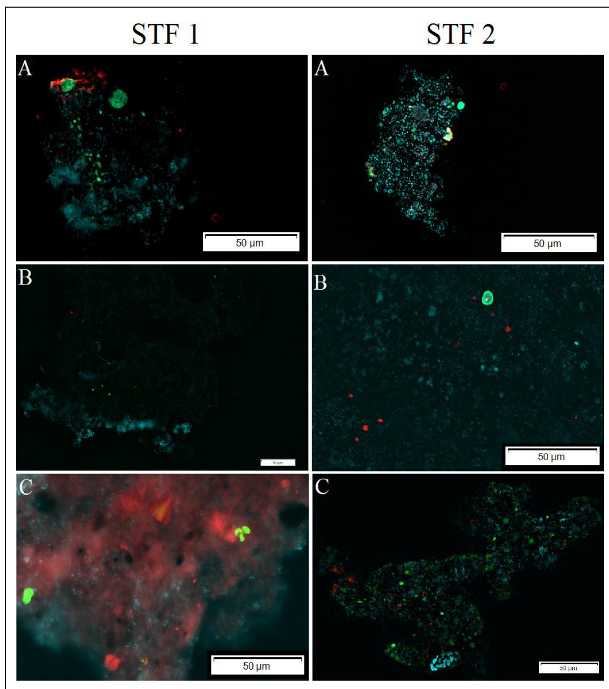
Figure 5.2. Identification by Fluorescence in situ Hybridization (FISH) of dominant microbial populations present in layers L_0 to L_2 in the STF reactors. All scale bars are 50 \mu\text{m} and the blue color indicates DAPI as general DNA stain. (A) The green color indicates ammonia-oxidizing organisms hybridized with NSO190 probe and red color indicates Anammox bacteria hybridized with AMX 820 probe; (B) The green color indicates nitrite oxidizing organisms hybridized with NIT 3 probe and red color indicates Anammox bacteria hybridized with AMX 820 probe; (C) The green color indicates ammonia-oxidizing organisms hybridized with NSO190 and NSO1225 probes and red color indicates nitrite oxidizing organisms with Nit 3, NSM 156 and Ntspa 662 probes.
