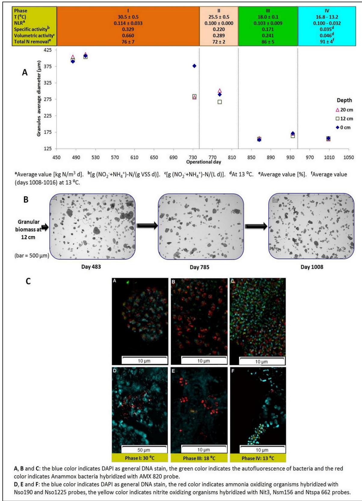
Figure 3.4. Granule size and microbial population variation in the Anammox SBR.
