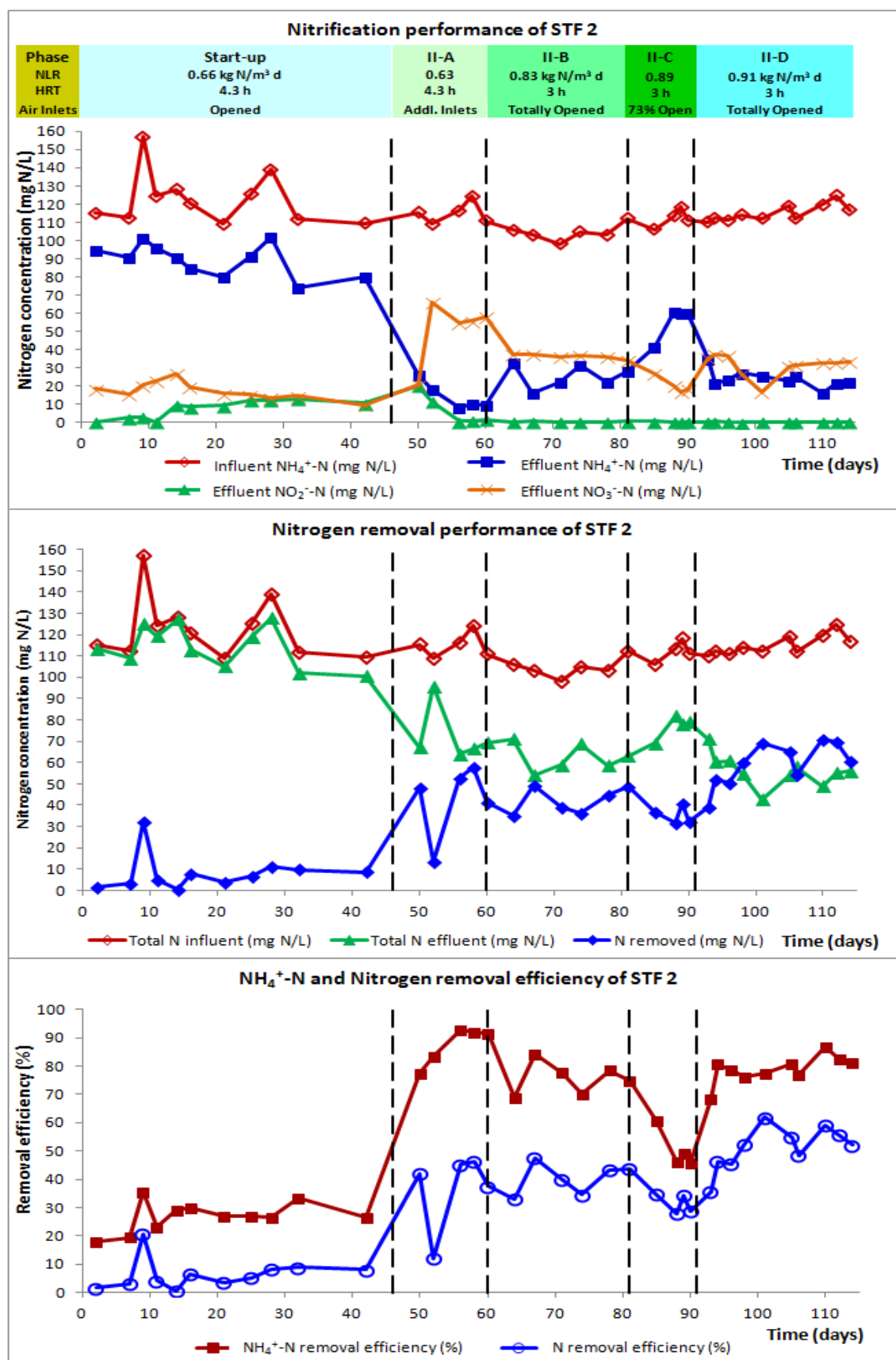
Figure 5.4. \text{NH}_4^+\text{-N} removal performance of STF-2.
