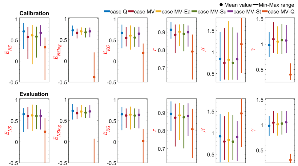
Figure 2. Statistics of model performance for streamflow. The best score of all the metrics is 1. The dots give the mean score, and the bars represent the min-max range of values for 11 streamflow gauges. The colors correspond to the model calibration cases.
