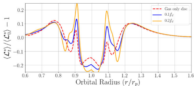
Figure 8. Radial profile of the azimuthally averaged ‘mixed’ key functions for a dust and gas disc with dust fractions of f_d = 0.1, 0.2 and Stokes number, St = 0.01 . The kinematic viscosity is set to \nu = 5 \times 10^{-7} and the evolution of the disc has reached t = 100 orbits. We see that large peaks have formed at the location of the gap edges showing the growth of the ‘mixed’ key function compared to initial.
