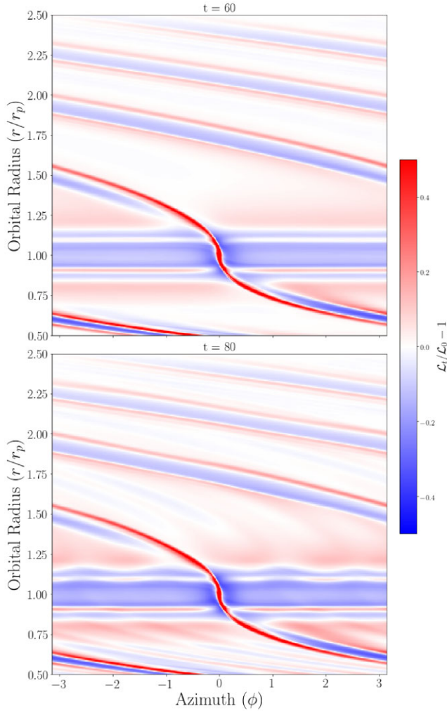
Figure 3. Key function plot for a gaseous disc with Neptune-sized planet embedded at 1r_p after t = 60, 80 orbits. The kinematic viscosity is, \nu = 10^{-7} and the gap edges interior ( r = 0.9r_p ) and exterior ( r = 1.1r_p ) to the planet has triggered the RWI generating a number of vortices which are more pronounced exterior to the planet.
