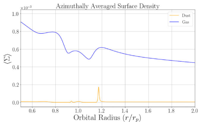
Figure 12. Radial profile of the azimuthally averaged surface densities for the dust (orange) and gas (blue) after t = 70 orbits. The dust evolution shows a sharp peak building at the outer pressure bump before the instability is triggered at around t = 78 .
