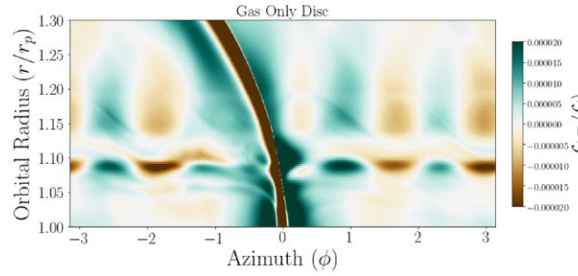
Figure 24. Typical structure of linear evolution of gas-only RWI. 2D plot of the non-axisymmetric part of the gas-only key function at t = 96 orbits with kinematic viscosity, \nu = 2.5 \times 10^{-7} . We see the formation of vortices exterior to the outer gap edge at r = 1.15r_p .
