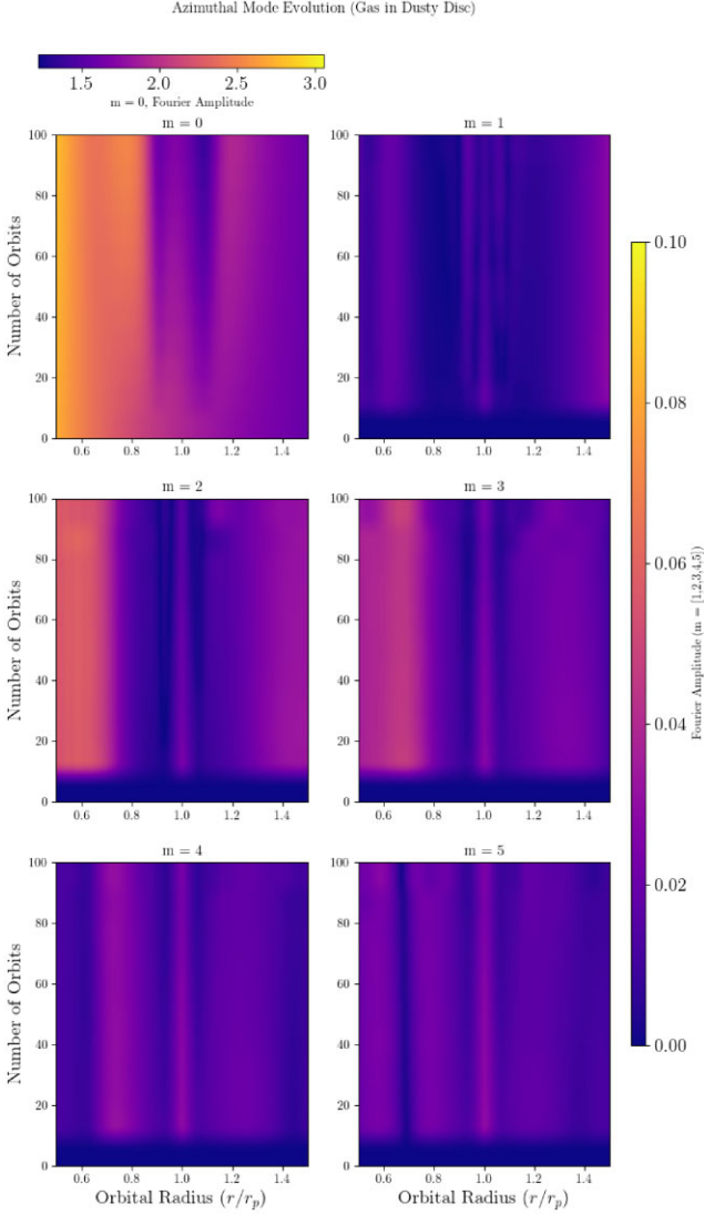
Figure 16. Time-evolution of the Fourier amplitudes of modes, m = 0-5 , for the gas in a Neptune planet embedded dusty disc with dust fraction f_d = 0.01 , St = 0.2 , and \nu = 5 \times 10^{-7} . The evolution of the Fourier amplitudes for all modes shows little variance in the region of the dusty ring location until t = 80 when the RWI is triggered, growing in amplitude from the outer gap edge and dusty ring location.
