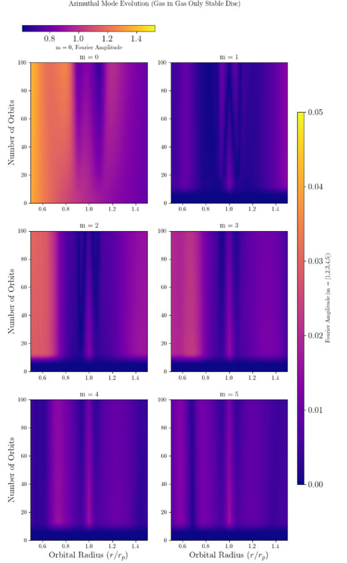
Figure 17. Time-evolution of the Fourier amplitudes of modes, m = 0-5 for the gas in a Neptune planet embedded gaseous disc with \nu = 1 \times 10^{-6} . In this disc, the gas is stable up to t = 100 , showing no features of instability growth in the outer pressure bump.
