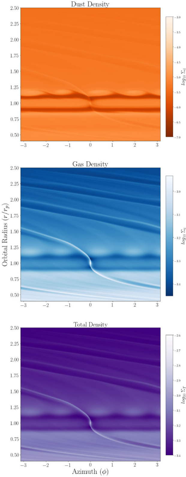
Figure 6. 2D density plots for the dust (top panel), gas (middle panel), and total (bottom panel) of a Neptune planet-embedded disc at t = 90 orbits. The dust fraction is set to f_d = 0.01 , Stokes number, St = 0.01 , and kinematic viscosity, \nu = 10^{-7} . We see that the dust from the outer ring is accumulated quickly into the vortices generated by the gap edge triggering the RWI.
