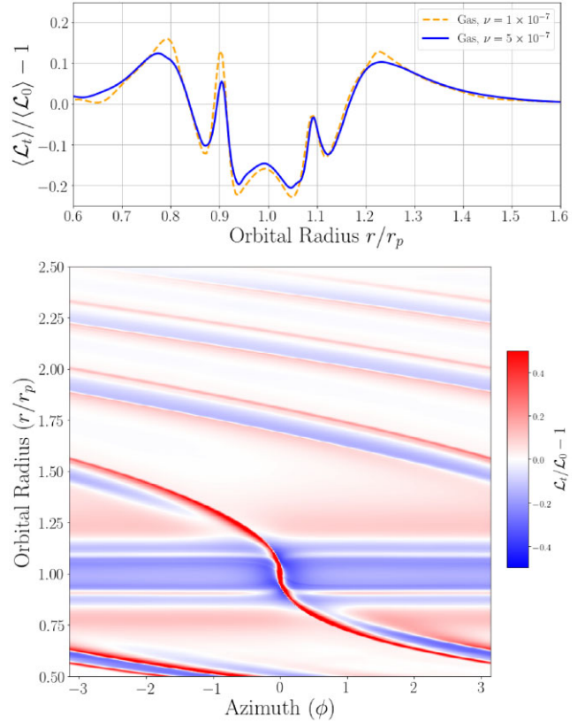
Figure 4. Radial profile of the azimuthally averaged key function (top panel) for stable (solid blue line) and unstable (dotted orange) gaseous discs. 2D key function plot (bottom panel) for a gaseous disc with Neptune-sized planet embedded at 1r_p after t = 100 orbits. The kinematic viscosity is set to \nu = 5 \times 10^{-7} . In this case, the kinematic viscosity is large enough to suppress the onset of the RWI during its evolution as shown in the bottom plot with a smooth gap edge interior and exterior to the planet, however, it is not as indicative in the radial profile of the key function compared to the lower viscosity case which goes unstable.
