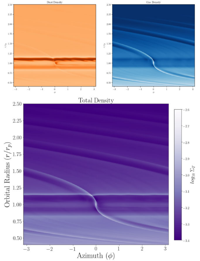
Figure 19. Density plots for dust (top left panel), gas (top right panel), and total (bottom panel) of the Neptune planet-embedded disc with dust fraction, f_d = 0.1 and Stokes number, St = 0.1 . The evolution of the disc is at t = 50 orbits. The dust ring formed exterior to the planet is smooth with vortices starting to be generated in the gap that the Neptune planet has carved for the dust phase which affects the gas phase and total density with weak spiral arms being launched through the disc.
