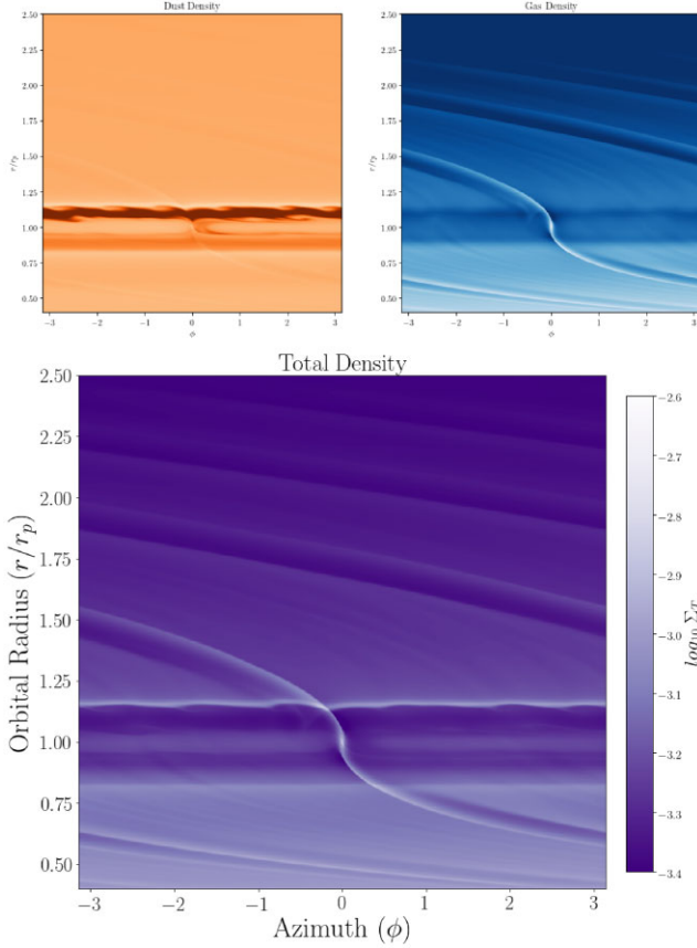
Figure 20. Density plots for dust (top left panel), gas (top right panel), and total (bottom panel) of the Neptune planet-embedded disc with dust fraction, f_d = 0.1 and Stokes number, St = 0.1 . The evolution of the disc is at t = 60 orbits. The dust ring has triggered the RWI at its location after the gap edges became unstable closer to the planet. Compared to previous setup, this indicates addition of dust makes the disc even more prone to the RWI.
