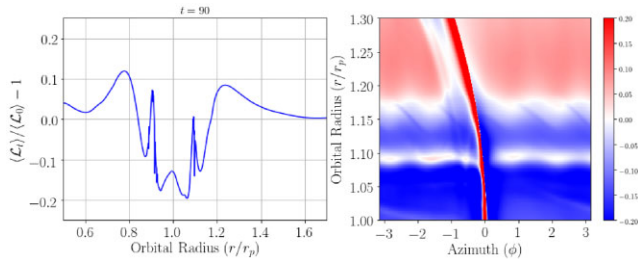
Figure 23. Radial profile of the azimuthally averaged key function (left panel) and 2D key function plot (right panel) for the gas phase of the disc. The dust fraction is set to f_d = 0.01 , Stokes number, St = 0.2 , and kinematic viscosity, \nu = 5 \times 10^{-7} . The 2D plot shows how the gas phase of the disc is affected by the dusty ring triggering the RWI through generation of vortices.
