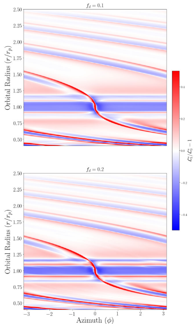
Figure 9. ‘Mixed’ key function plot for dust and gas disc with dust fractions, f_d = 0.1 (top panel) and 0.2 (bottom panel) with Stokes number, St = 0.01 for both cases. The evolution of the disc has reached t = 100 orbits. The gap edges interior and exterior to the planet remain generally stable during its evolution with the dusty rings being largely undisturbed.
