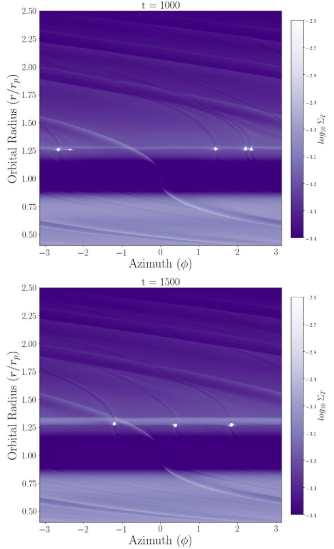
Figure 28. Total density plots for the disc at t = 1000 (top panel) and t = 1500 (bottom panel) with dust fraction, f_d = 0.01 , Stokes number, St = 0.2 , and kinematic viscosity, \nu = 5 \times 10^{-7} . A secondary wider dusty ring is shown to be forming exterior to the locations of the vortices which have merged into three distinct points.
