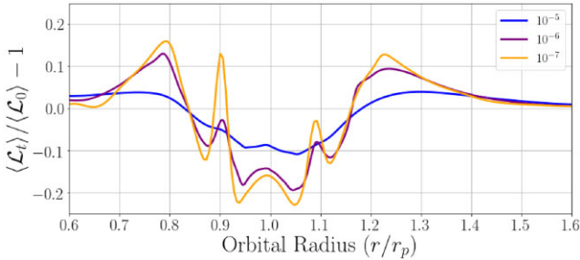
Figure 2. Radial profile of the azimuthally averaged key functions for \nu \in [10^{-5}, 10^{-6}, 10^{-7}] . The lower viscosity setups have a larger peak at the location of the gap edges ( r = 0.9r_p, 1.1r_p ) which lead to development of the RWI.
