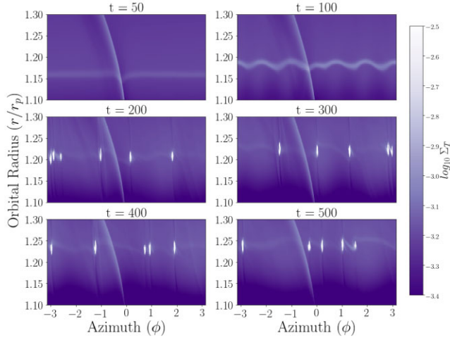
Figure 27. Total density plots for region exterior to a Neptune planet that is embedded in a dust and gas disc with dust fraction, f_d = 0.01 , Stokes number, St = 0.2 , and kinematic viscosity, \nu = 5 \times 10^{-7} . The plots shown are the time-evolution of the disc, t \in [50, 100, 200, 300, 400, 500] .
