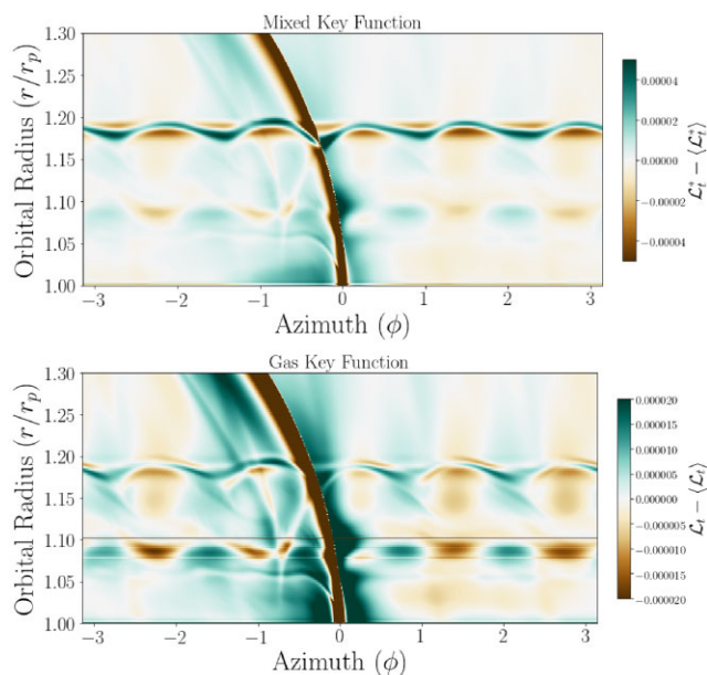
Figure 25. 2D plot of the non-axisymmetric part of the mixed (top panel) and gas (bottom panel) key function at t = 100 orbits. The dust fraction is set to f_d = 0.01 , Stokes number, St = 0.2 , and kinematic viscosity, \nu = 5 \times 10^{-7} . We see the formation of vortices similar to the linear evolution of the gas-only RWI at the outer gap edge with additional structures at the location of the ring.
