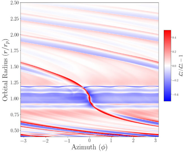
Figure 14. 2D ‘mixed’ key function plot at t = 100 orbits for a dust and gas disc with Neptune-sized planet-embedded disc. The dust fraction is set to f_d = 0.01 , Stokes number, St = 0.2 , and kinematic viscosity \nu = 5 \times 10^{-7} .
