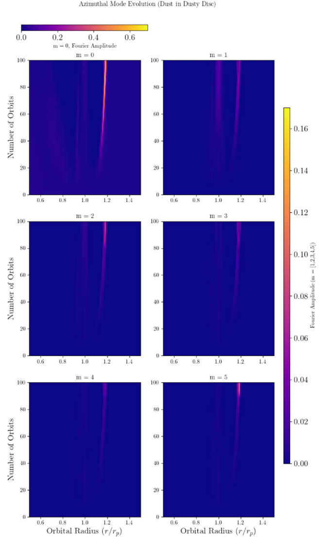
Figure 15. Time-evolution of the Fourier amplitudes of modes, m = 0-5 , for the dust in a Neptune planet embedded dusty disc with dust fraction f_d = 0.01 , Stokes number, St = 0.2 , and \nu = 5 \times 10^{-7} . The growth of the Fourier amplitudes at r/r_p = 1.2 dominates where the location of the thin dusty ring is formed and triggers the RWI.
