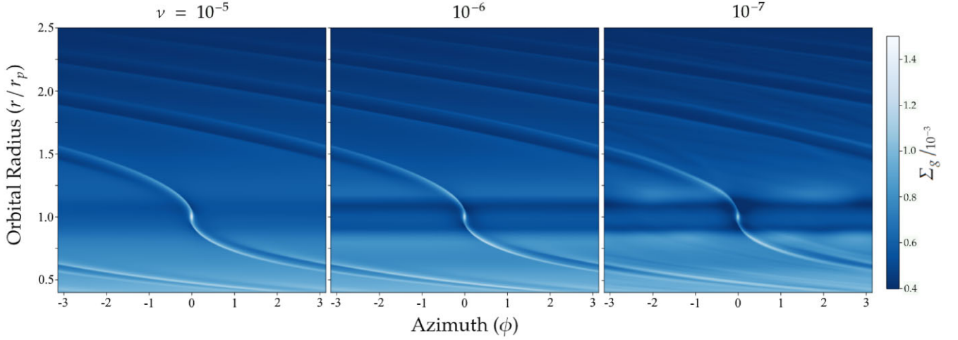
Figure 1. Density plots for a gaseous disc with a Neptune-sized planet embedded at 1r_p after t = 100 orbits. The kinematic viscosity is varied, \nu \in [10^{-5}, 10^{-6}, 10^{-7}] from the left to right panels. RWI has developed in the rightmost plot with the lowest kinematic viscosity at the inner and outer rings and has caused vortices to emerge, destabilizing the gas rings and gap edges ( r = 0.9, 1.1r_p ).
