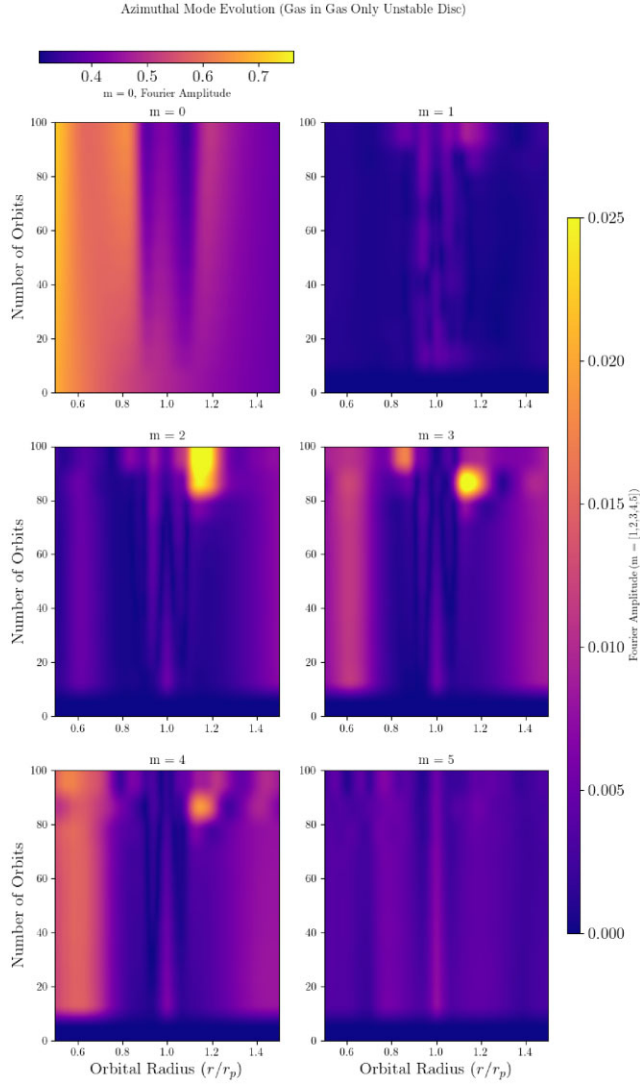
Figure 18. Time-evolution of the Fourier amplitudes of modes, m = 0 – 5 for the gas in a Neptune planet embedded gaseous disc with \nu = 1 \times 10^{-7} . For this disc, the gas triggers the RWI by t = 100 orbits and we see clear features in the plots for modes 2–4 indicating the growth of the instability.
