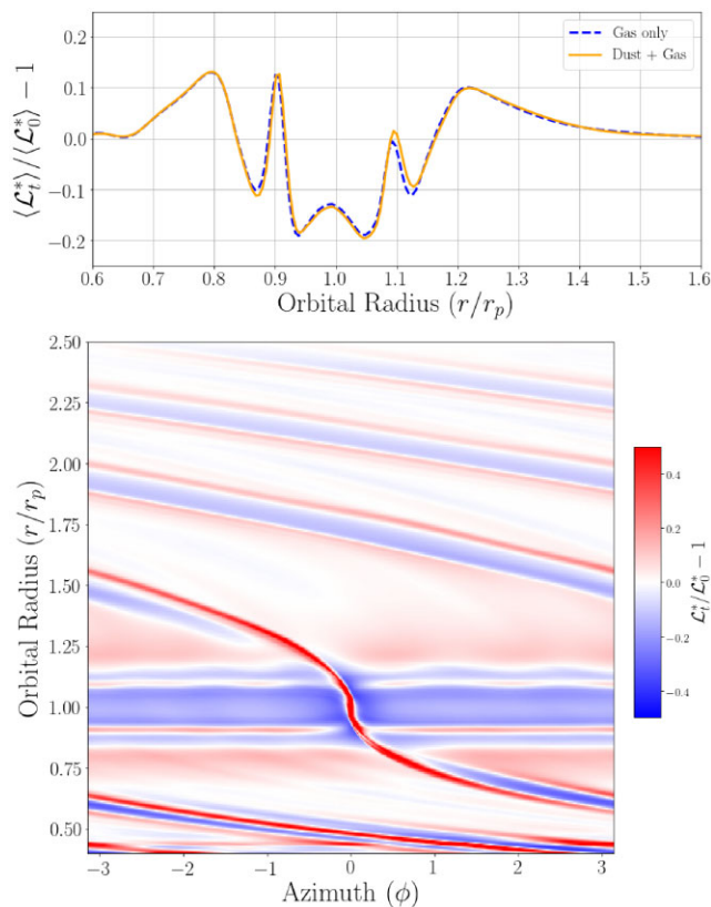
Figure 5. Radial profile of the azimuthally averaged ‘mixed’ key function (top panel) for dust and gas (solid orange) and radial profile of gas-only key function (dotted blue). 2D key function plot (bottom panel) for the dust and gas disc with Neptune-sized planet embedded at 1r_p after t = 80 orbits. The dust fraction is set to f_d = 0.01 , Stokes number, St = 0.01 and kinematic viscosity, \nu = 10^{-7} . With the addition of dust the gap edges interior and exterior still trigger the RWI which generates vortices but has little differences compared to the gas-only case.
