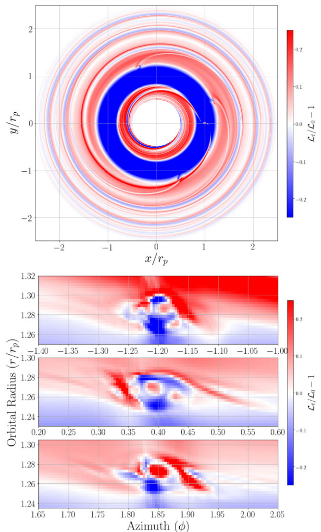
Figure 26. Polar plot of the ‘mixed’ key function (top panel) and zoom in of the three vortices that have formed after t = 1500 orbits for a Neptune planet-embedded disc with dust fraction, f_d = 0.01 and Stokes number, St = 0.2 . We see that the centres of the vortices have accumulated a large amount of dust and the inner structure of the vortex is chaotic.
