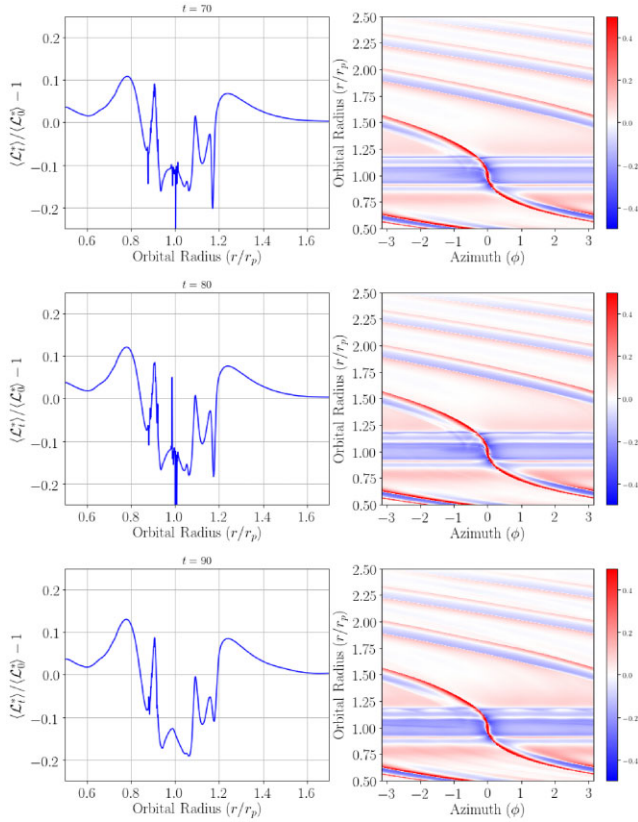
Figure 22. Time-evolution of the ‘mixed’ key function for a Neptune planet embedded with dust fraction, f_d = 0.01 and Stokes number, St = 0.2 at t \in [70, 80, 90] orbits (top, middle, and bottom panels). Perfect coupling is introduced at t = 78 through modifying the collision rate. We see that the RWI is responsible for the vortices generated at the dusty ring’s location rather than drag instabilities.
