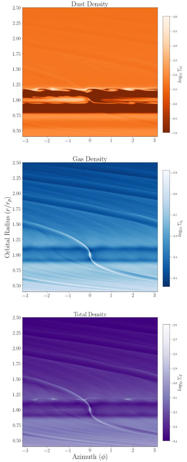
Figure 7. 2D density plots for the dust (top panel), gas (middle panel), and total (bottom panel) of a Neptune planet-embedded disc at t = 90 orbits. The dust fraction is set to f_d = 0.01 , Stokes number, St = 0.1 , and kinematic viscosity, \nu = 10^{-7} . The thin dusty ring built exterior is destabilized by vortices at the gap edge and material is accumulated into vortex centres, which causes weak spiral density waves to be launched from the vortices.
