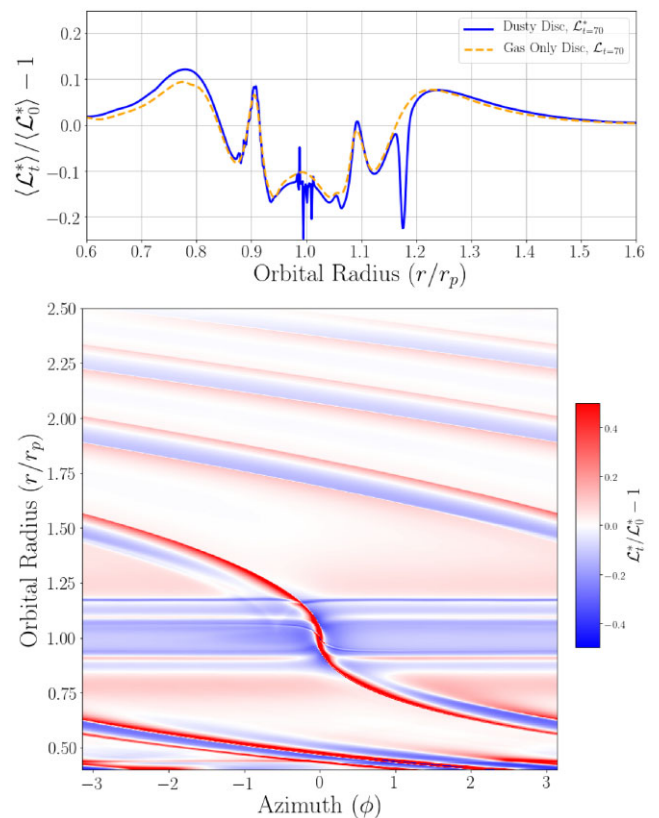
Figure 13. Radial profile of the azimuthally averaged ‘mixed’ key function of a dust and gas disc (blue line) compared to gas key function for a gas-only disc (dashed orange line) (top plot) and 2D key function plot (bottom panel) for a dust and gas disc with Neptune-sized planet embedded at 1r_p after t = 70 orbits. The dust fraction is set to f_d = 0.01 , Stokes number, St = 0.2 , and kinematic viscosity, \nu = 5 \times 10^{-7} . The radial profile shows a sharp minimum at the dust ring’s location and indicates that the width of the extremum is an important factor which indicates location of regions prone to the RWI.
