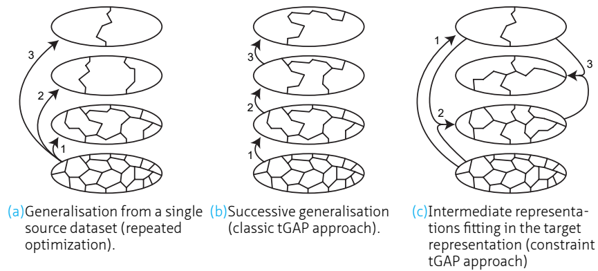
FIGURE 3.6 Approaches to create a sequence of LoDs from (Haunert et al., 2009).
