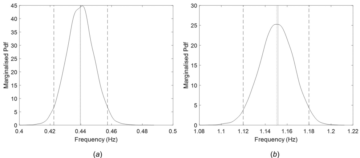
Fig. 11 Probability density functions of modal parameters given equivalent dispersion parameter value \delta_s = 0.098 : ..... mean value; ——— 95th percentile; ..... deterministic value: (a) first natural frequency and (b) second natural frequency
