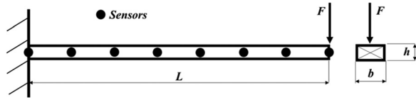
Fig. 12 Schematic representation of the cantilever system
