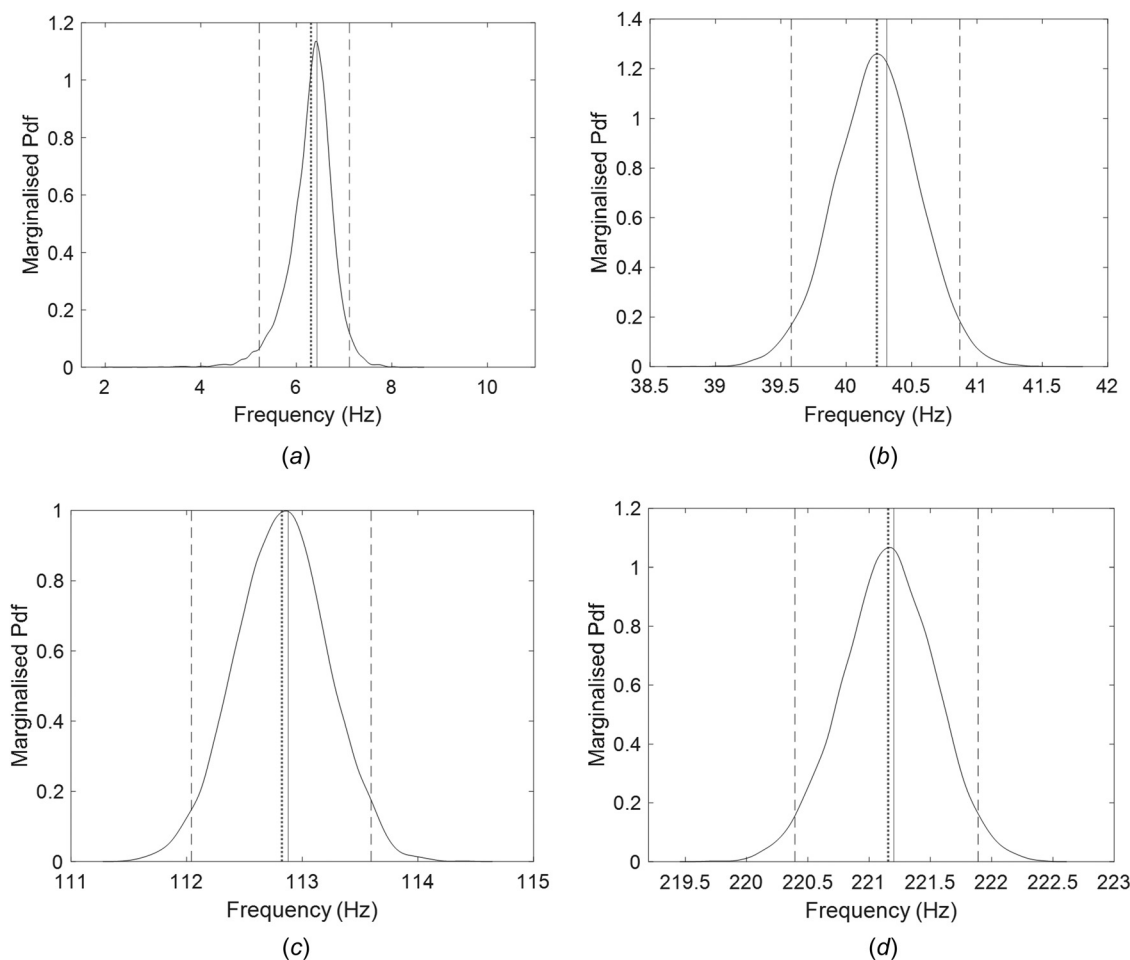
Fig. 16 Probability density functions of natural frequencies for a dispersion value: \delta_S = 0.075 : ..... mean value; ——— 95th percentile; ..... deterministic value: (a) first natural frequency, (b) second natural frequency, (c) third natural frequency, and (d) fourth natural frequency
