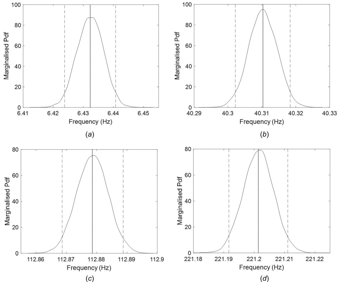
Fig. 13 Probability density functions of natural frequencies for a dispersion value: \delta_S = 0.001 : ..... mean value; ——— 95th percentile; ..... deterministic value: (a) first natural frequency, (b) second natural frequency, (c) third natural frequency, and (d) fourth natural frequency
