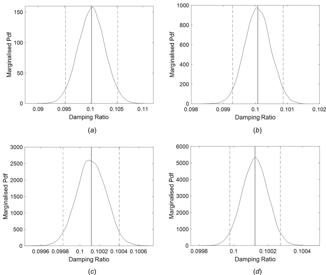
Fig. 14 Probability density functions of damping ratios for a dispersion value: \delta_S = 0.001 : ..... mean value; ——— 95th percentile; ..... deterministic value: (a) first damping ratio, (b) second damping ratio, (c) third damping ratio, and (d) fourth damping ratio
