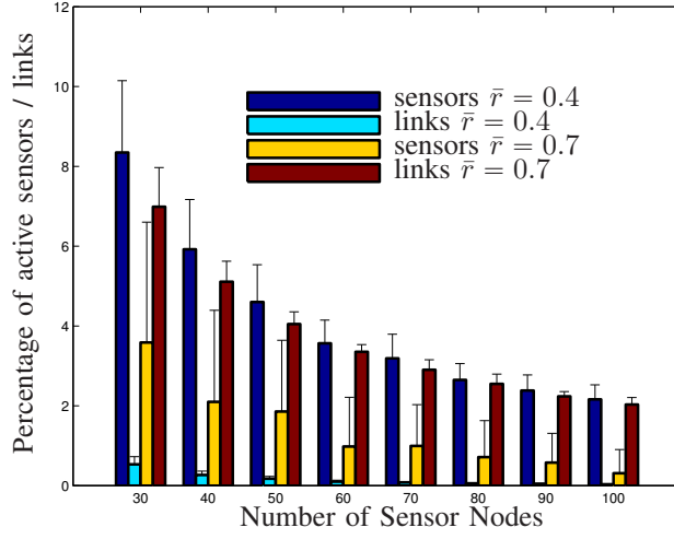
Figure 11: Average percentage of active sensors and links and its standard deviation for m = 2 and for different amount of sensors and \bar{r} .
