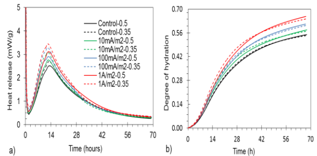
Figure 3. Heat released (a) and degree of hydration (b) as function of time for cement paste with w/c 0.5 and 0.35.
