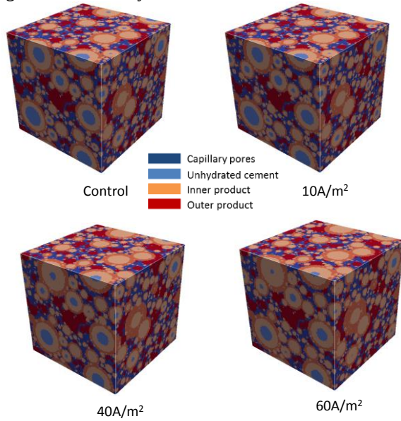
Figure 11. 3D microstructure of cement hydration at different level electrical current flow with water-to-cement ratio 0.5.
