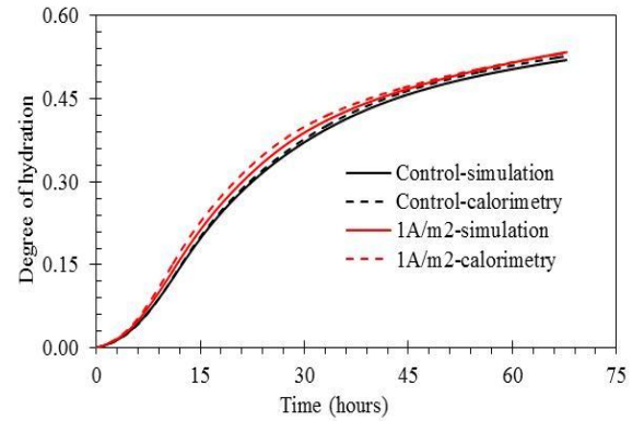
Figure 7. Simulation of degree of hydration as function of time for cement paste with w/c 0.5 and validation with experimental data from calorimetry tests.
