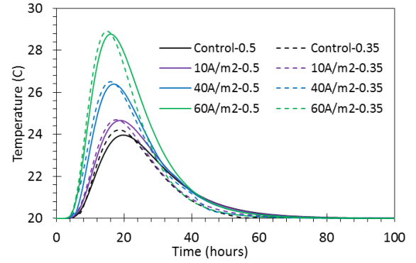
Figure 6. Relationship between applied electrical current density and temperature development of cement paste.
