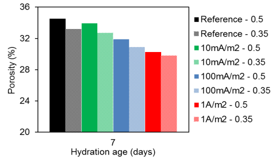
Figure 5. Total porosity development of cement paste
