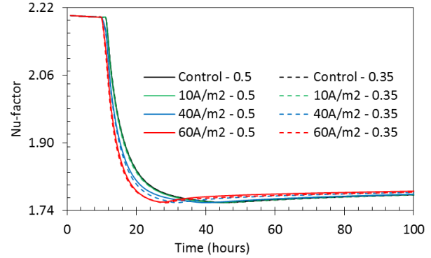
Figure 10. Nu-factor development of paste as function of time
