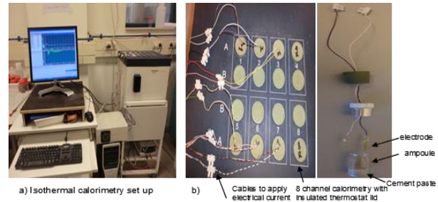
Figure 2. (a) Isothermal calorimeter (TAM-Air-314) used to measure heat release of cement paste; (b) Schematic pictures of the holders for “under current” regime (Series C).
