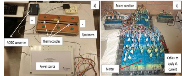
Figure 1. Experimental set-up for measurements of temperature increase in cement paste and mortar specimens due to electrical current flow (Series A) (a) and experimental set up of electrical current flow through mortar specimens in sealed condition (Series B) (b).
