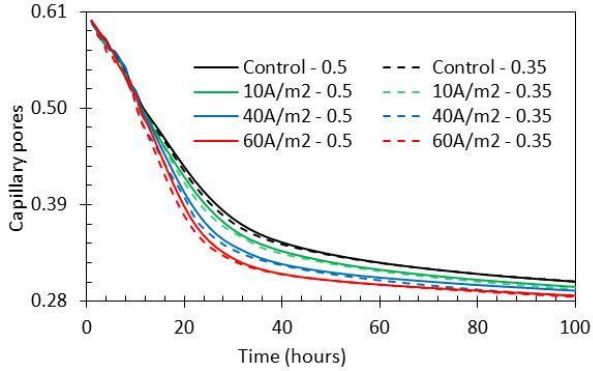
Figure 9. Capillary pores development of cement paste in condition of electrical current flow as function of time
