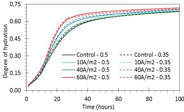
Figure 8. Degree of hydration of cement paste with different level electrical current density as function of time.
