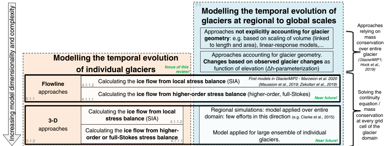
Figure 10. Schematic evolution of dimensionality and ice-dynamical representation in ice-dynamical glacier evolution studies (IDGES) performed on individual glaciers (left side, orange box) and large-scale IDGES (at regional and global scales, right side, blue box). The links between studies performed on individual glaciers and those performed at large scales highlight how techniques that were typically used for individual glaciers are now starting to be applied in large-scale IDGES. Gray numbers refer to the numbering of the sections in which the respective topics are addressed.
