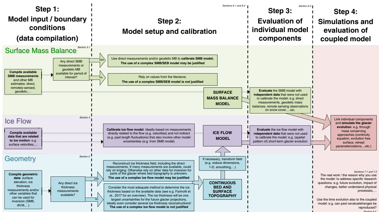
Figure 12. Schematic overview of steps to follow when deciding on model setup and experimental design for glacier evolution modeling. The procedure is meant as a general example and, depending on the available data and goal of the study, it may be advisable to deviate from this. Also note that a few aspects that can be important for specific cases (e.g., studies including glaciers with important frontal mass balance and debris cover) are not accounted for in this diagram.
