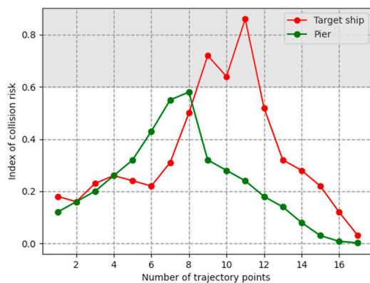
(c) The results detected by fuzzy theory based model
