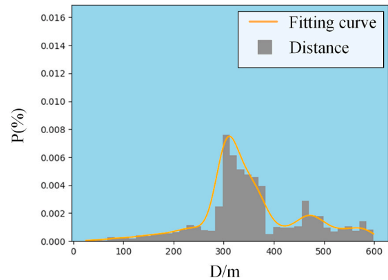
(b). Fitting curve of a region by KDE method
