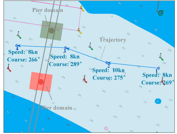
(b). The diagram of pier domains and trajectory
