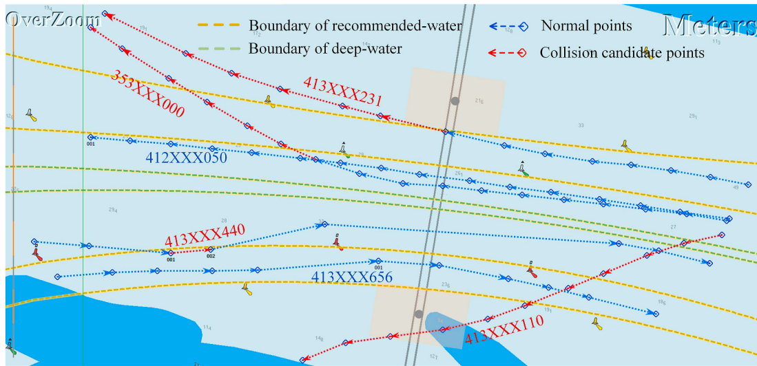
Fig. 22. Result of collision candidate detection with t_f = 30s
