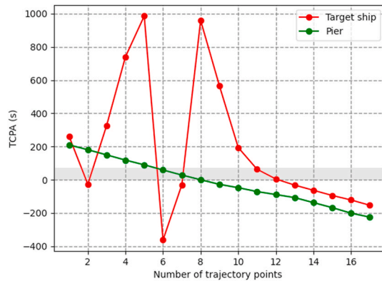
(a) The results of TCPA
