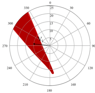
(b). Velocity space of the 9 th trajectory point
