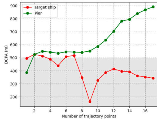
(b) The results of DCPA
