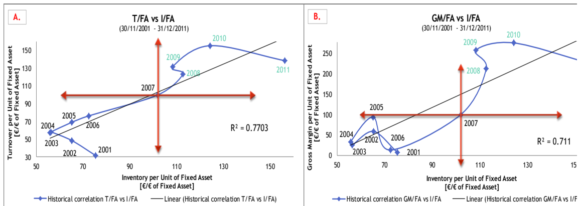
Figure 6. Level 1 - Quadrants visualisation in graphs A.) T/FA vs. I/FA B.) GM/FA vs. I/FA I/FA values indexed with respect to 2007
