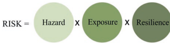
Fig. 1.4 Resilience-based risk analysis
