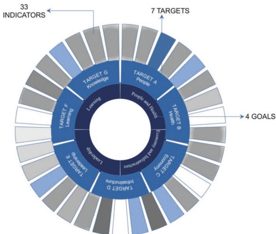
Fig. 1.6 Synthetized Sendai framework structure (adopted to ARUP, 2014)
