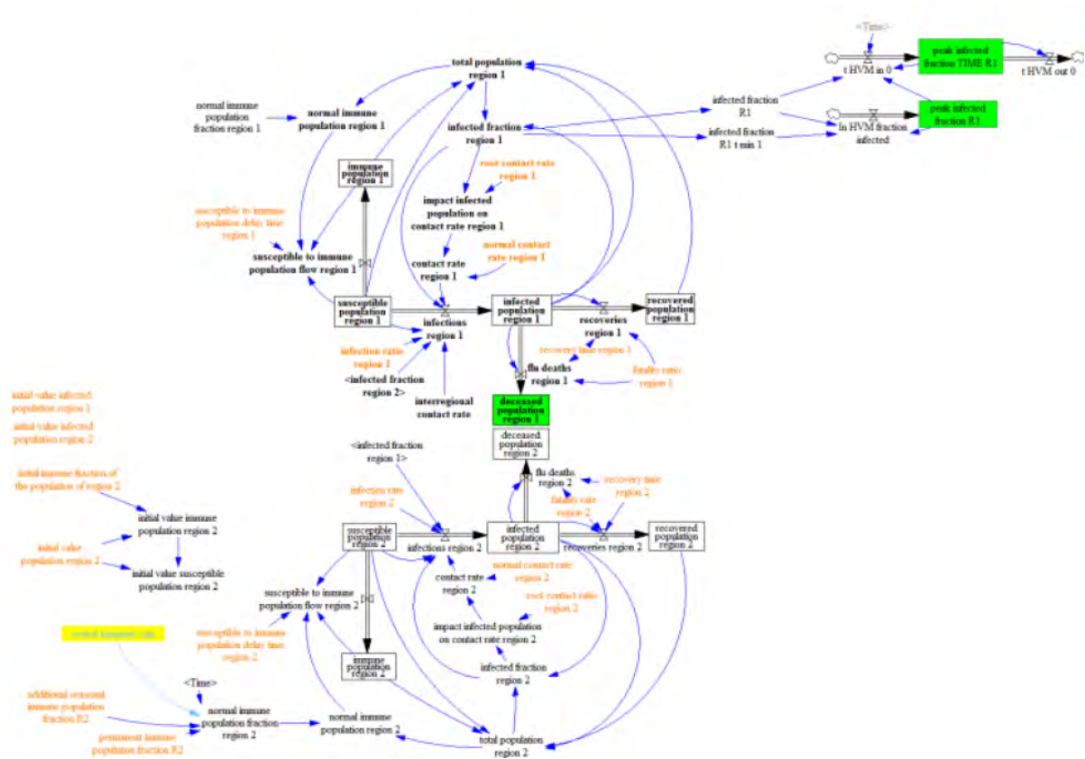
Figure 5: Stock-flow structure of the flu model
