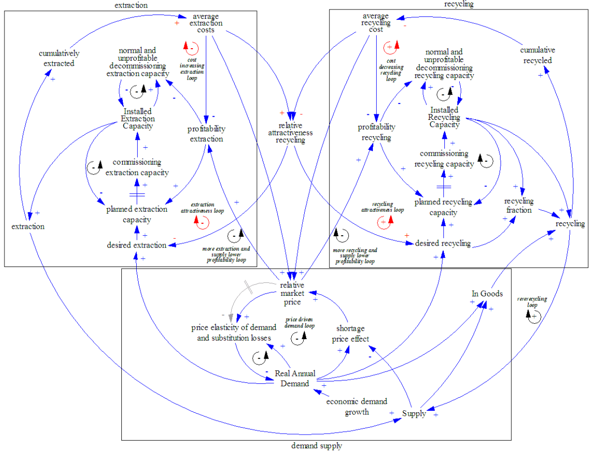
Figure 2: Main views and feedback loops of the SD simulation model
