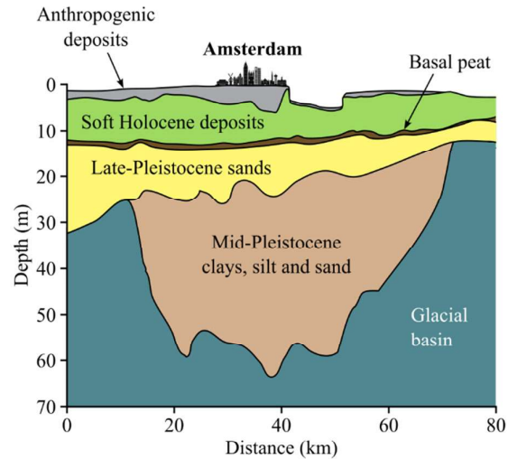
Fig. 3. Geological cross-section of Amsterdam
