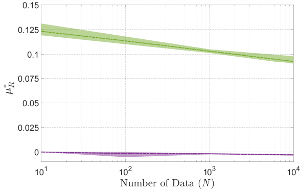
Fig. 2. Optimal values \mu_R^* acquired from Lyapunov functions via solving SOP 1 in (9a) (i.e., purple curve) and SOP 2 in (9b) (i.e., green curve).
