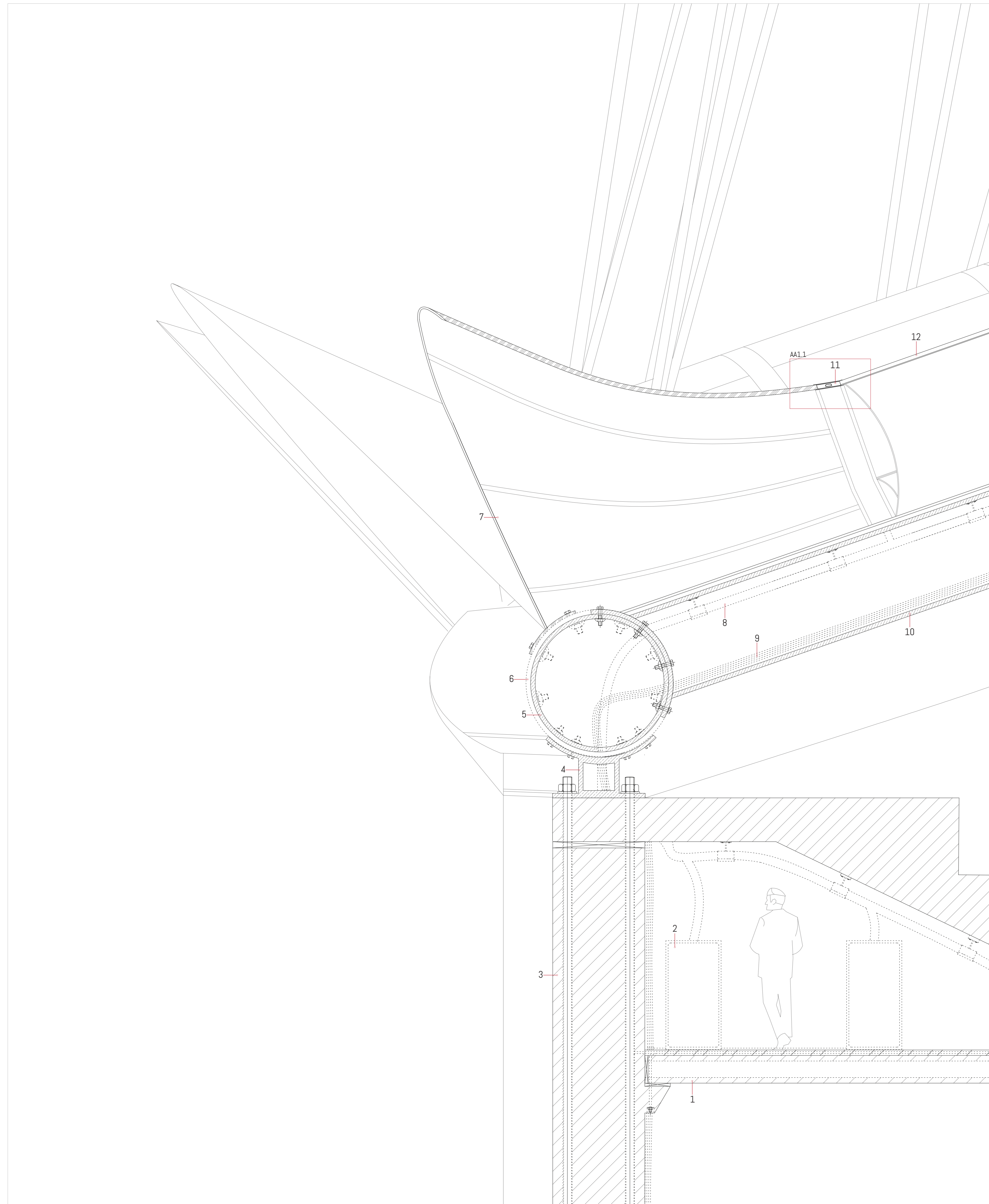
DETAIL AA1.1 1:5
