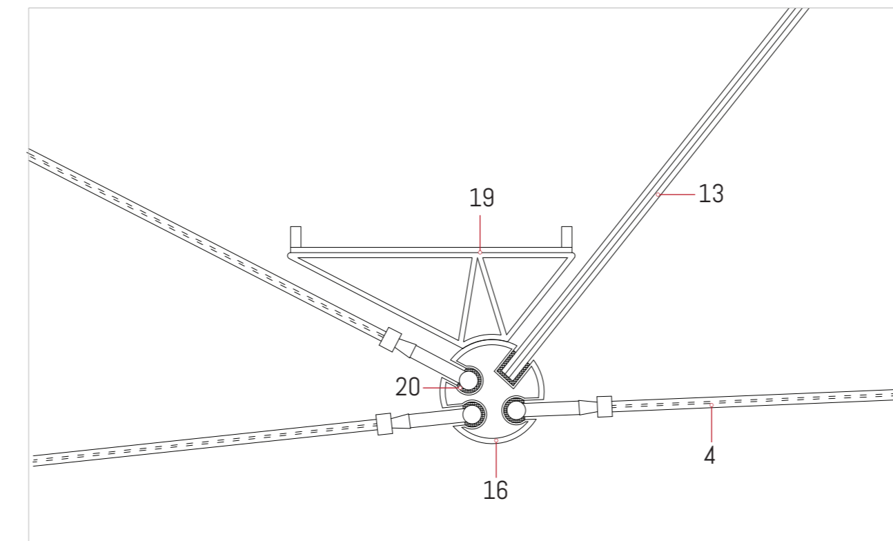
DETAIL BB3.1 1:5
