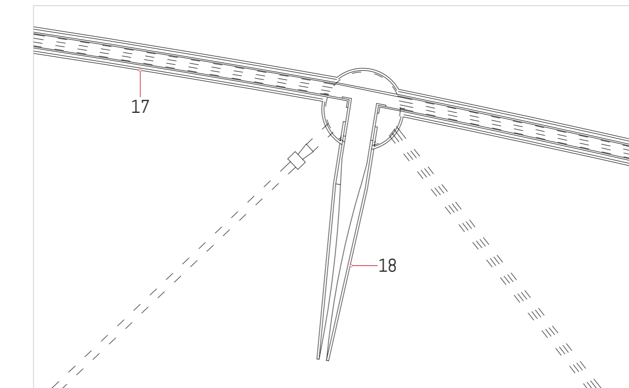
DETAIL BB3.2 1:5
