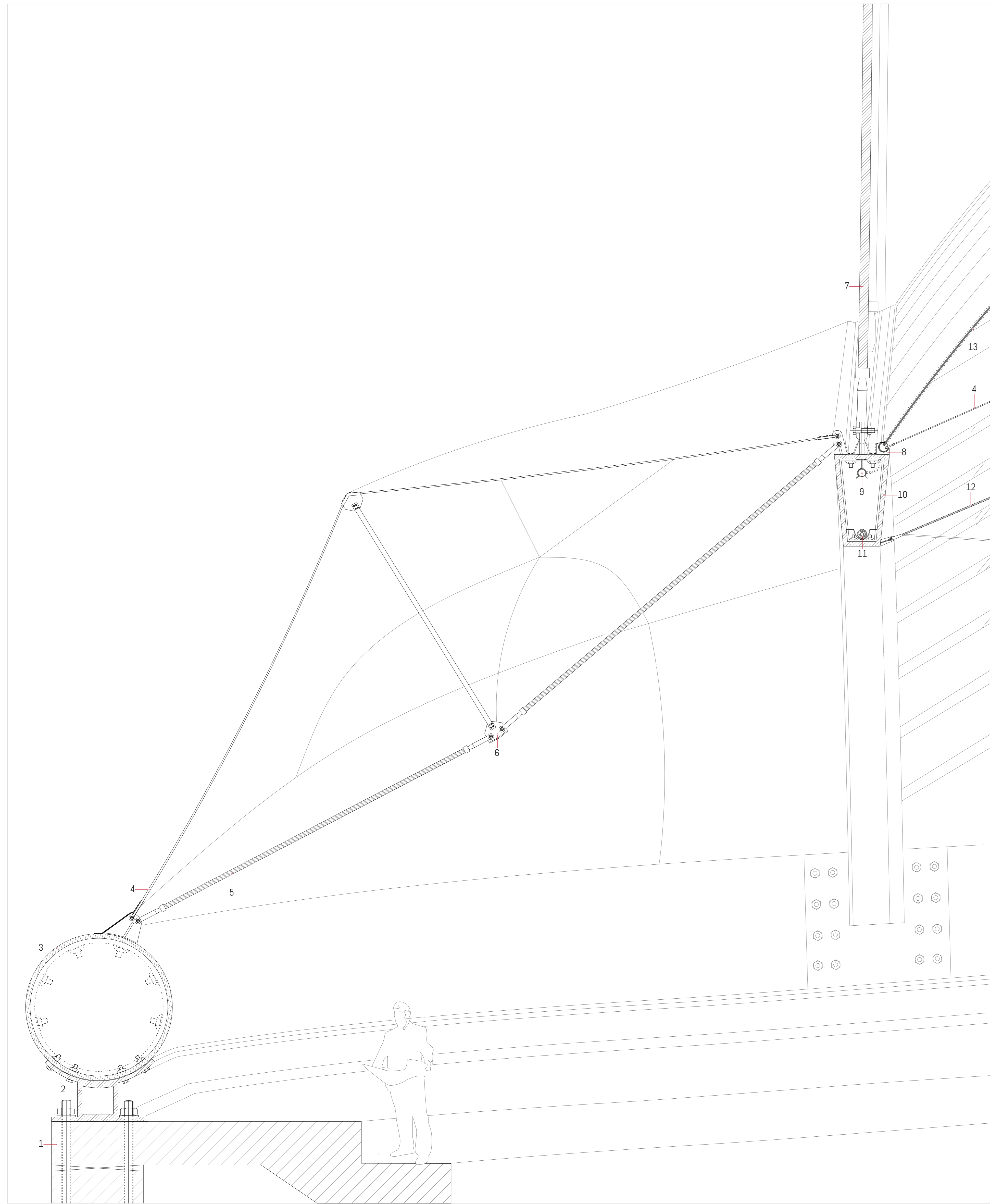
DETAIL BB1 1:20
