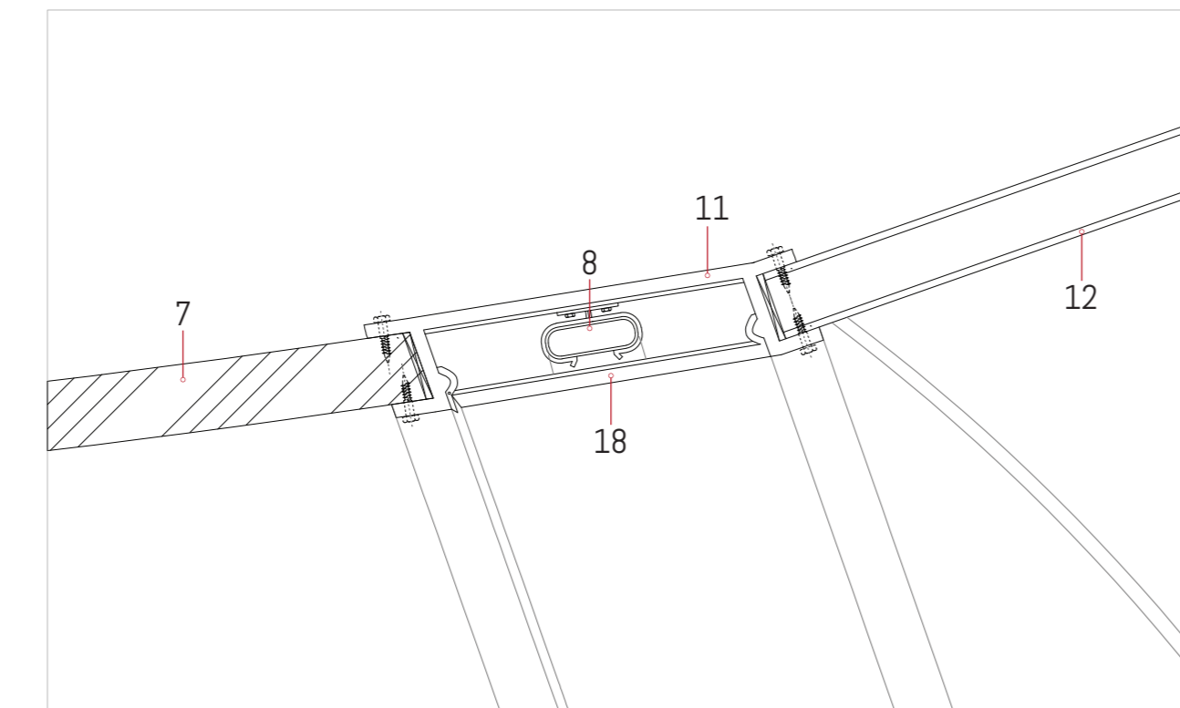
DETAIL AA1.1 1:5
