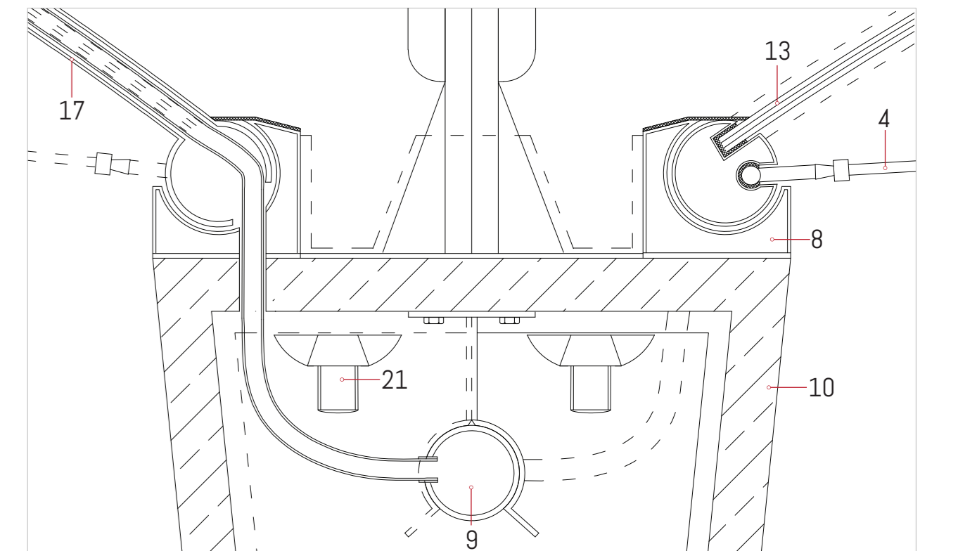
DETAIL BB3.3 1:5
