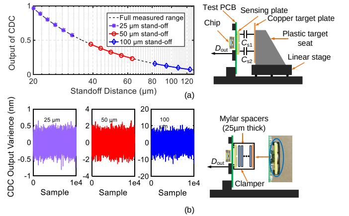
Fig. 9. Measured displacement transfer characteristics (a) and the outputs of the CDC (10,000 decimated samples) with different stand-offs along (b).
