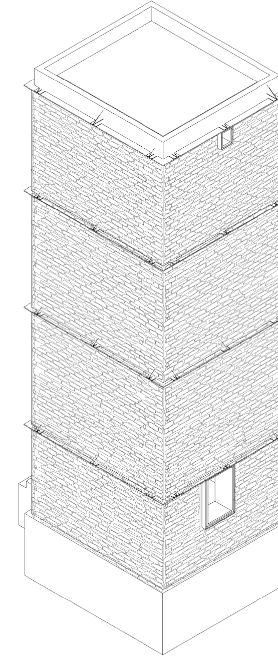
stage 6 stone facade infill thin layer of lime applied between the rocks by local craftsman, insulation and interior cladding
