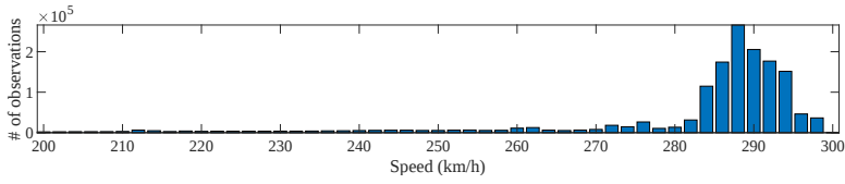
Figure 5.7: Number of observations distributed with inspection train speed.
