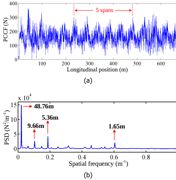
Figure 2.4: (a) The computed PCCF signal and (b) its power spectrum density (PSD).
