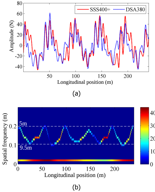
Figure 2.12: (a) Extraction results comparison and (b) CSWs spectrum in Case 2.
