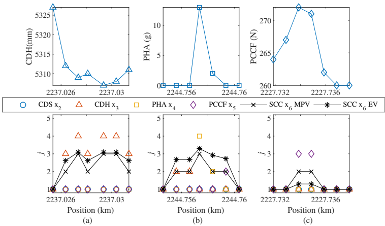
Figure 5.12: Three previous false alarms that are identified as medium risk or below ( j \leq 3 ) by the BN-based approach. The false alarms were previously triggered by the (a) CDH, (b) PHA and (c) PCCF data shown at the top, respectively. The data PIs and BN outputs using the most probable value (MPV) and the expected value (EV) are shown at the bottom.
