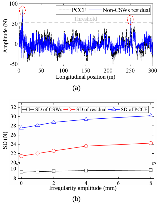
Figure 2.15: (a) The mean-removed PCCF measurement data and its non-CSW residual. (b) Comparisons of the standard deviations (SDs) of PCCF, CSWs and non-CSW residual with respect to the irregularity amplitude.
