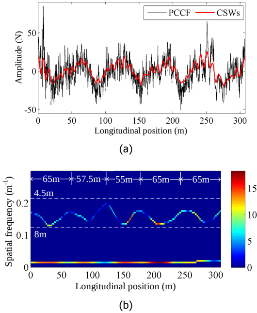
Figure 2.14: (a) The mean-removed PCCF measurement data comparing with its CSWs and (b) the CSWs spectrum of the PCCF in Case 3.
