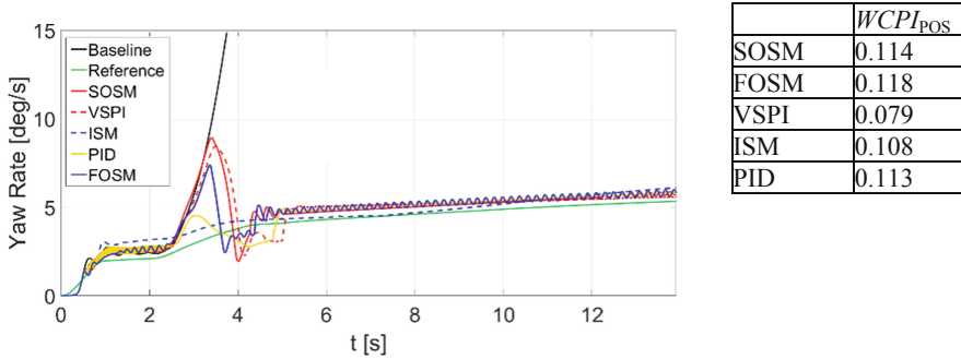
Fig. 5. Yaw rate diagrams and WCPI values for a power oversteering test.
