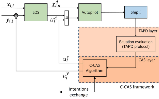
Fig. 1. Control scheme with the proposed C-CAS framework: U_i^d and \chi_{i,n}^d are desired thrust and course angle in the inertial coordinate frame \{n\} ; the control signals from CAS are cross-track offset, u_i^y , and speed modification, u_i^s .
