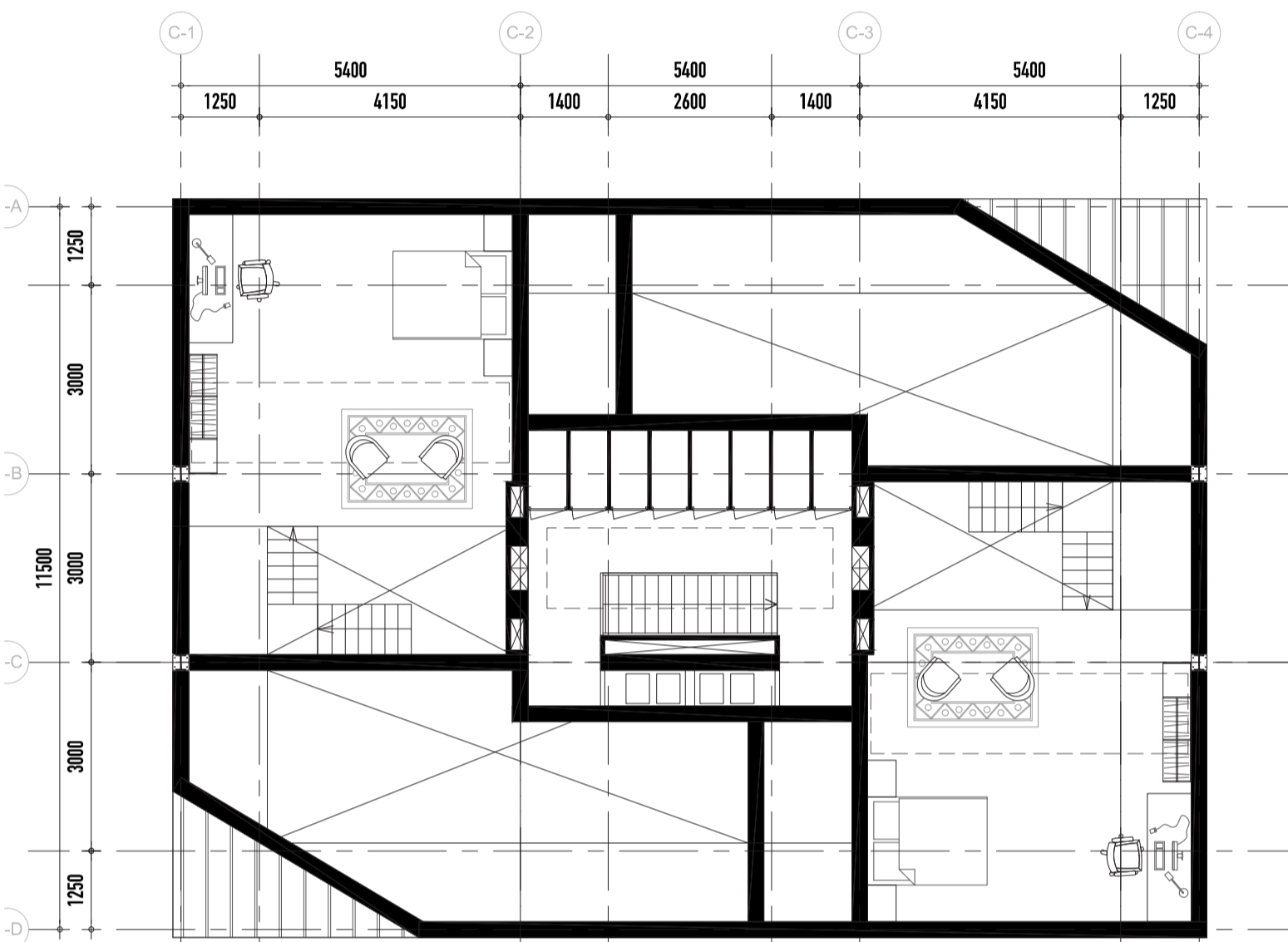
Mezzanine floor
