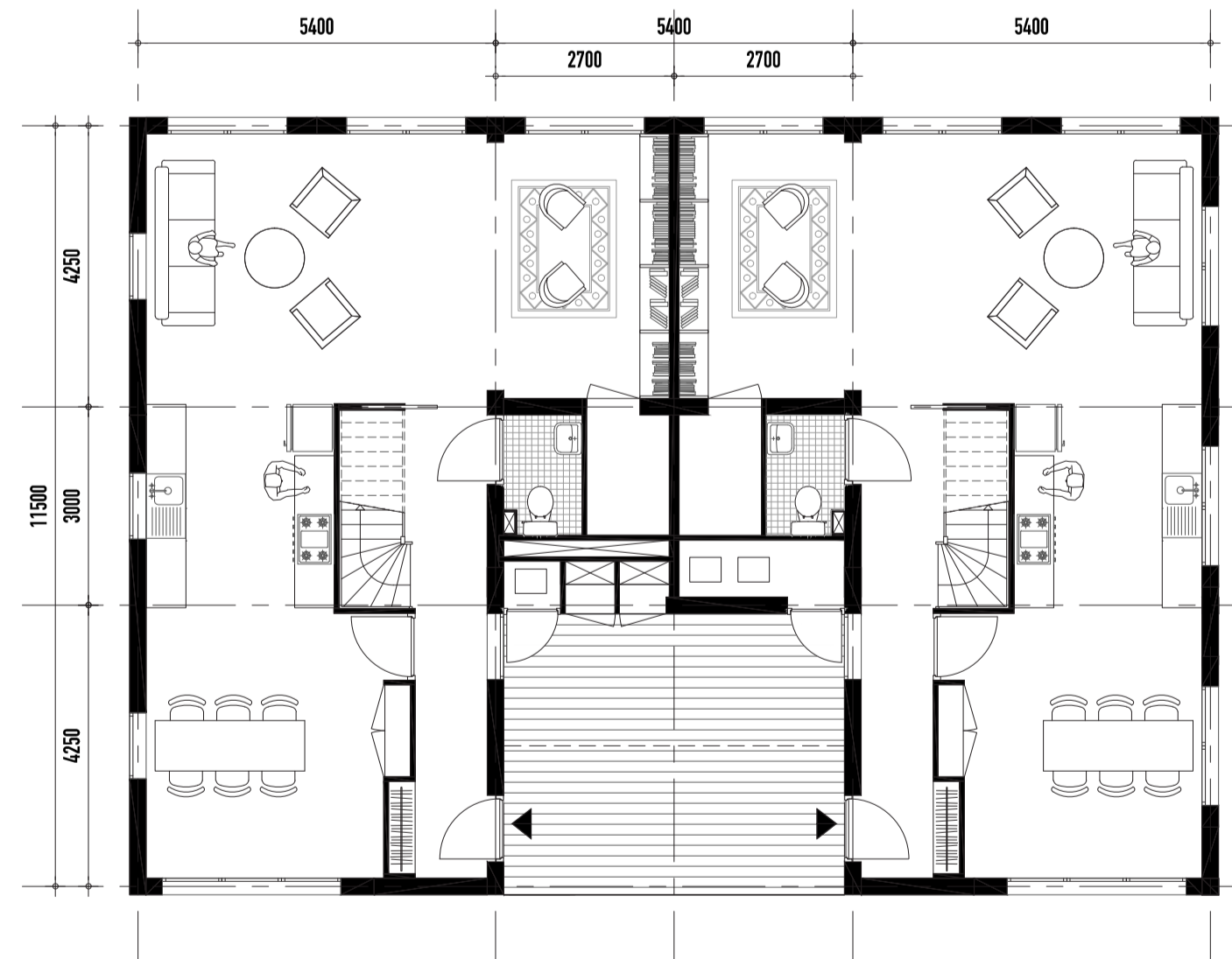
Lower floor
