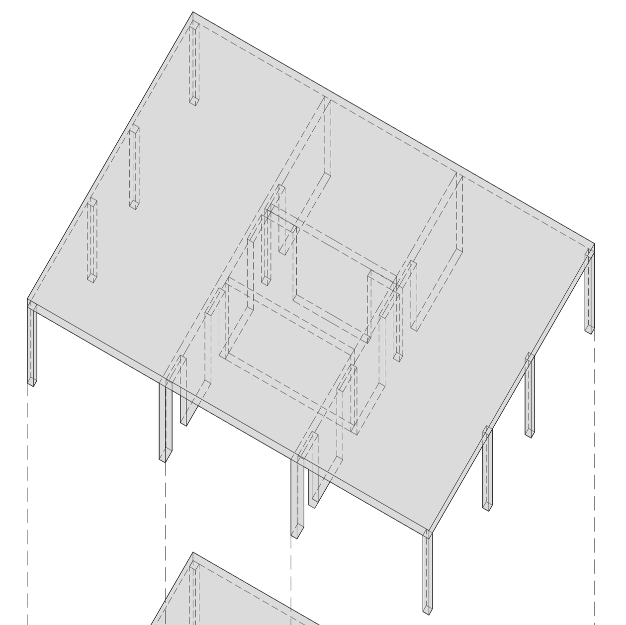
Upper floor
