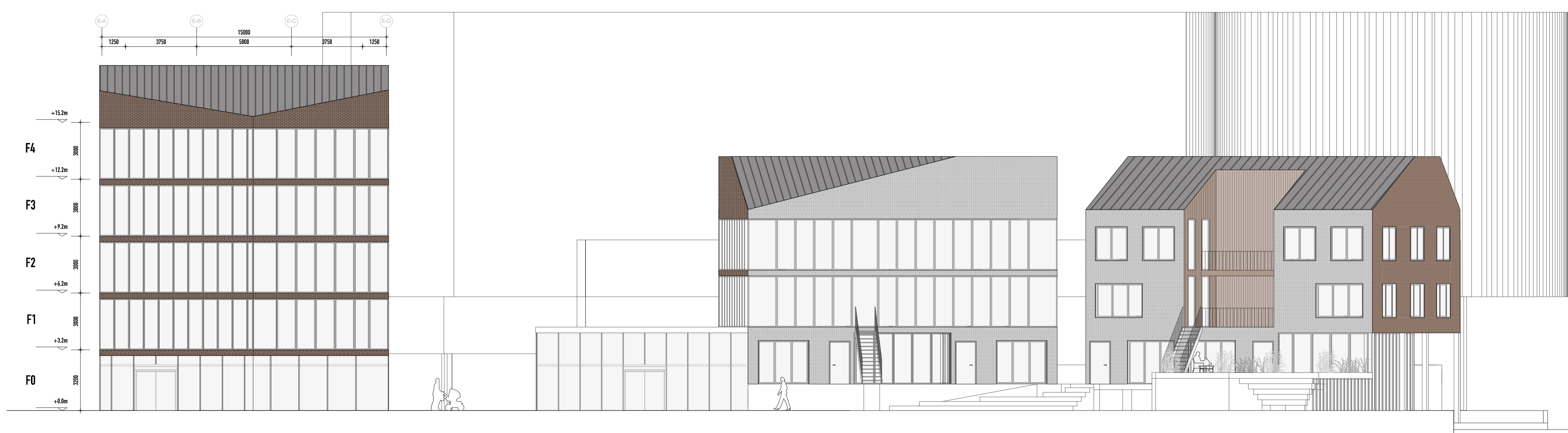
Section aa' 1:150
