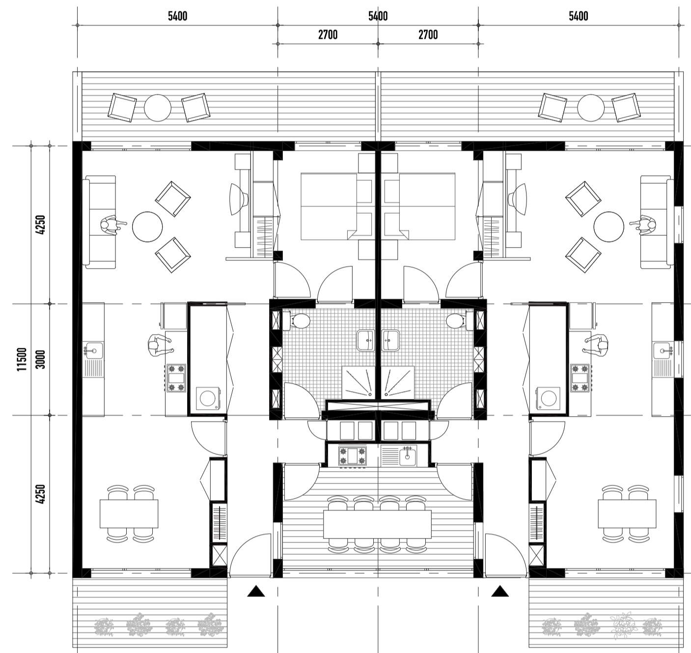
Plan 1: 100
