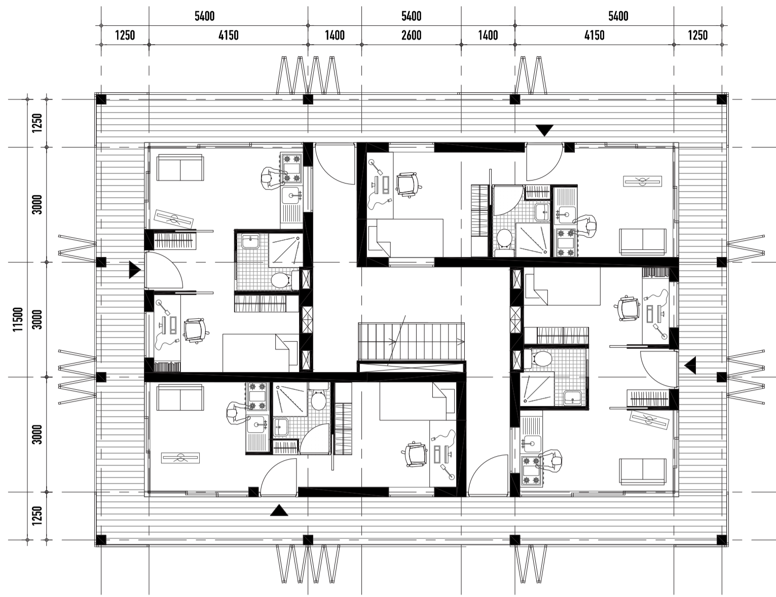
Plan 1: 100
