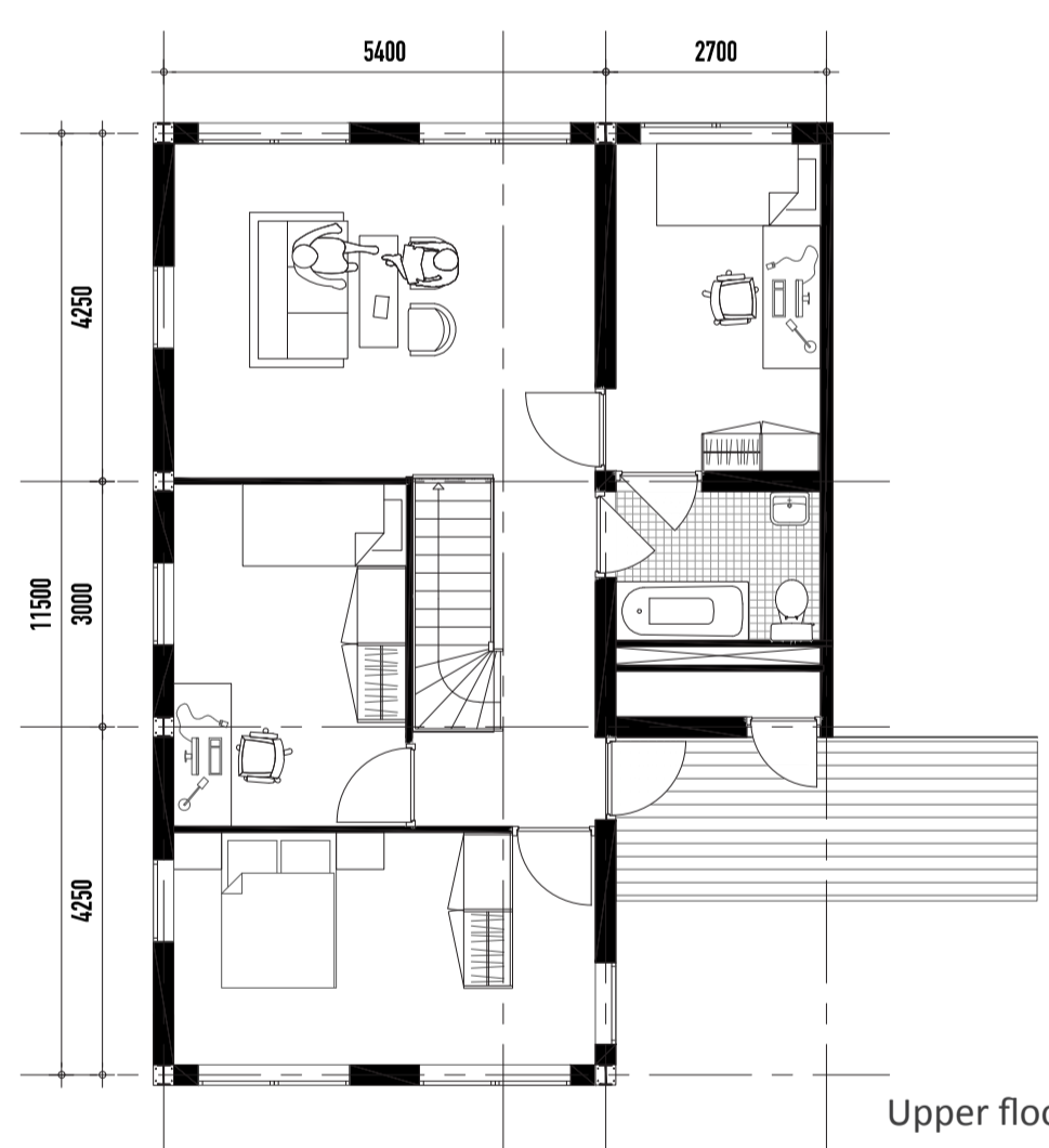
Upper floor
