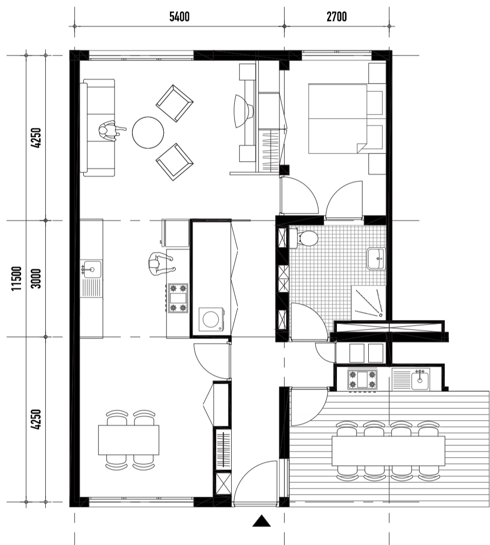
Unit plan 1: 100
