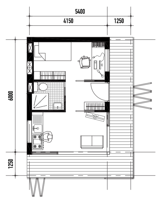
Unit plan 1: 100
