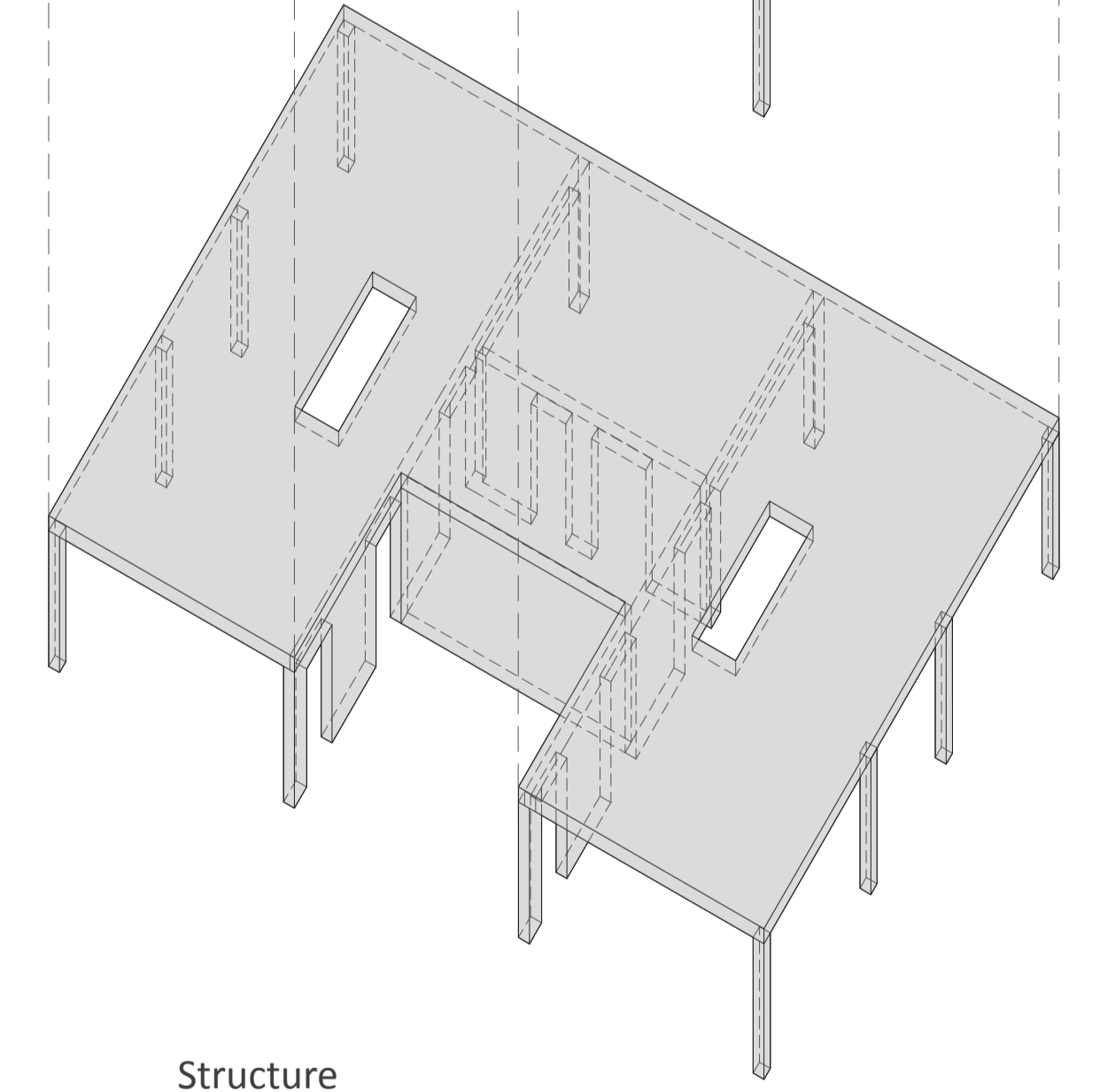
Structure
