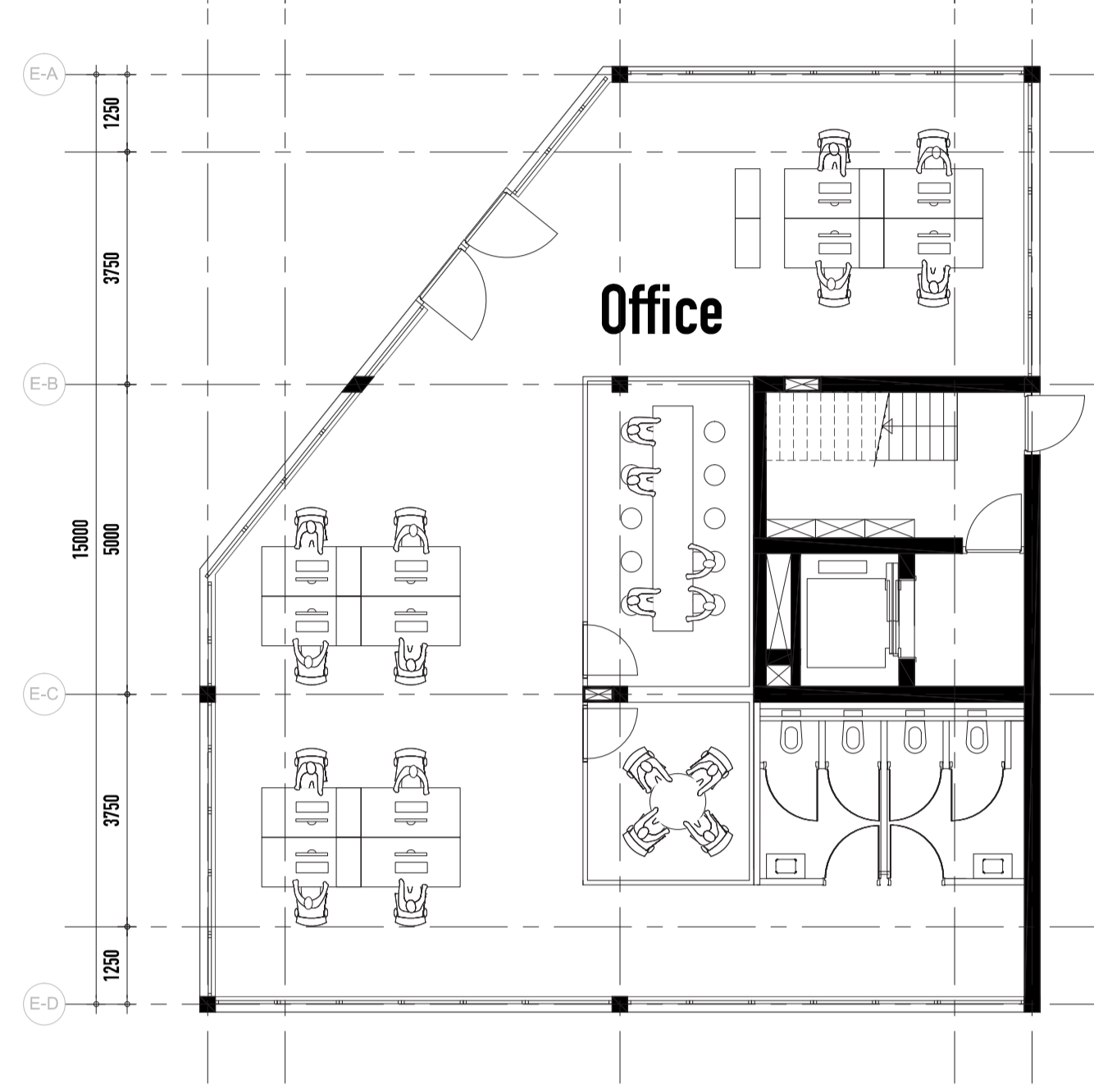
North block(E)_Plan 1 : 100
