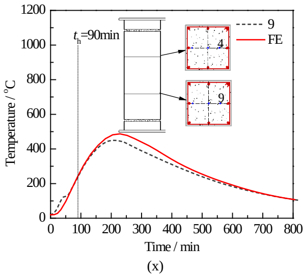
Fig.12 Measured and predicted cross-sectional temperatures of specimens: S200-45min: (a) steel tube; (b) and (c) reinforcement bars; (d) - (f) concrete; S200-90min: (g) steel tube; (h) and (i) reinforcement bars; (j) - (m) concrete; S250-45min: (n) steel tube; (o) and (p) reinforcement bars; (q) - (s) concrete; and S250-90min: (t) steel tube; (u) and (v) reinforcement bars; (w) - (y) concrete.
