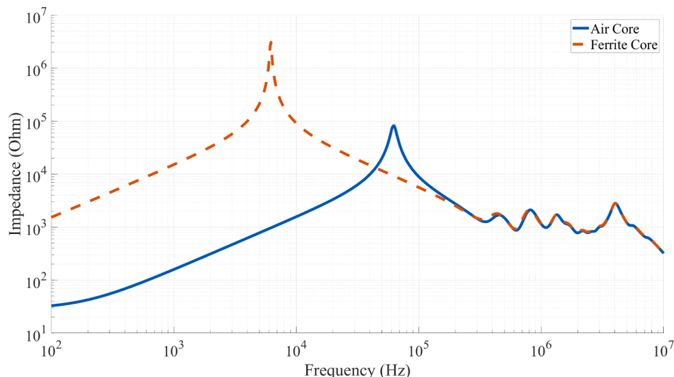
Fig. 11. Frequency response of the inductor with air and ferrite cores.
