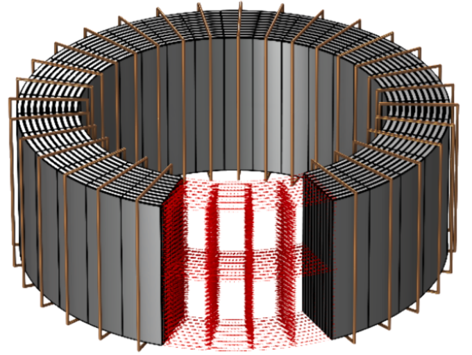
Fig. 2. The geometry of the laminated core.
