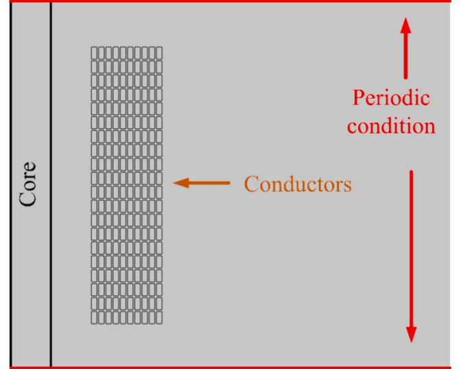
Fig. 5. The geometry of the winding used for the simulations.
