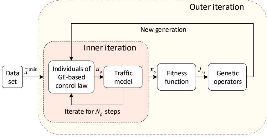
Figure 3.6: The diagram of Framework-2, where u_p is the control input generated by the parameterized control law, \mathbf{x}_p is the vector containing all the state information and control inputs that are used in the objective function (3.18), and J_{F2} is the optimized objective value of (3.18).
