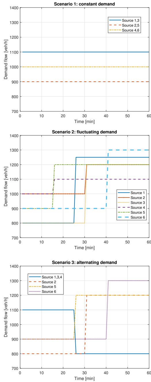
Figure 3.11: Demand profiles of the three scenarios used in the case study
