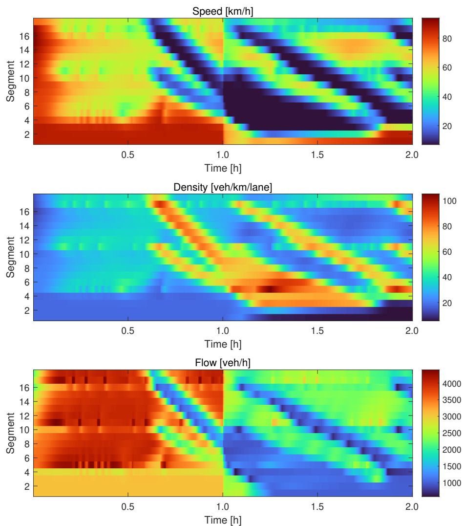
Figure 5.7: Traffic states of the freeway network during the simulation interval with the standalone PMPC controller for Scenario 1.
