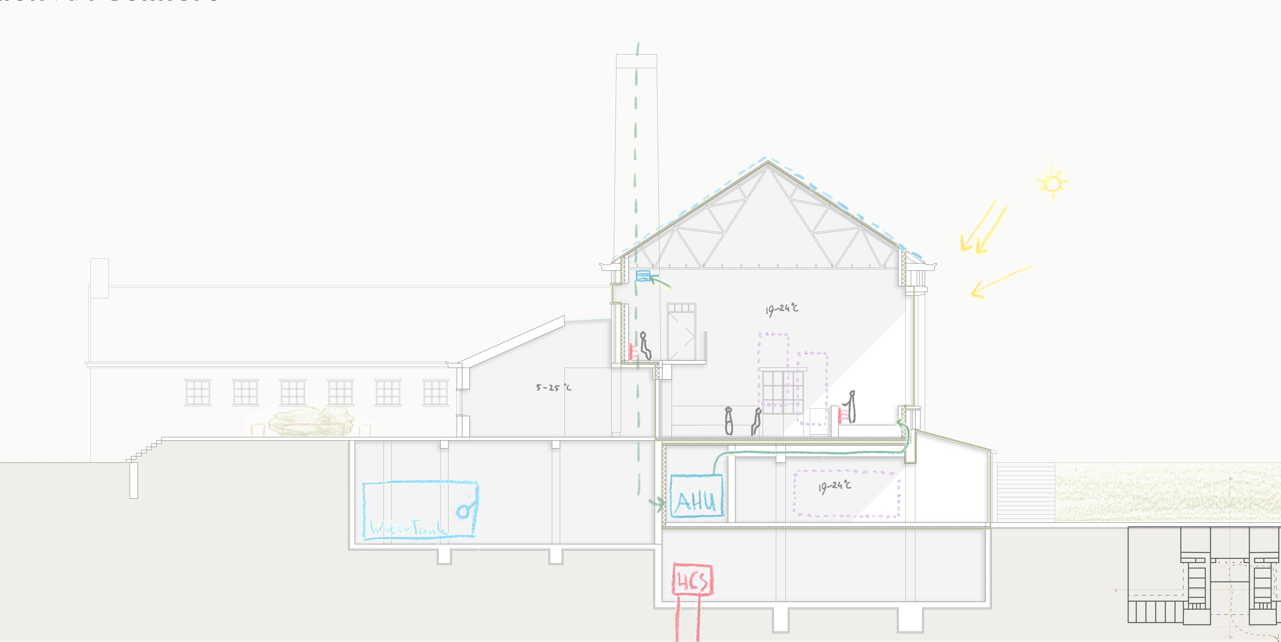
Section AA Comfort diagram
