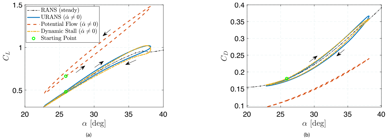
FIGURE 10 | Lift (a) and drag (b) coefficients versus the angle of attack of the RFD kite for the pitching motion of cycle 2 in Figure 4. Results from steady RANS, unsteady RANS, potential flow and semiempirical dynamic stall models are shown.
