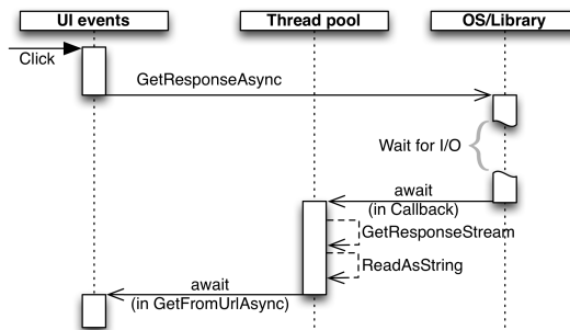
Figure 2: Where is the async/await code executing?
