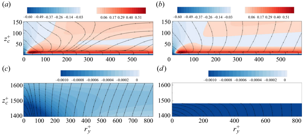
Figure 3. Near-wall (a,b) and outer (c,d) zoom of the fluxes of scale energy (black lines with arrows) in the compound space of spanwise scales and wall distances (\phi_{r_y}^+, \phi_{z_c}^+)(0, r_y^+, 0, z_c^+) and isocontours of the scale energy source \xi^+(0, r_y^+, 0, z_c^+) for a turbulent boundary layer (a,c) and a turbulent channel (b,d) at Re_\tau = 1500 .
