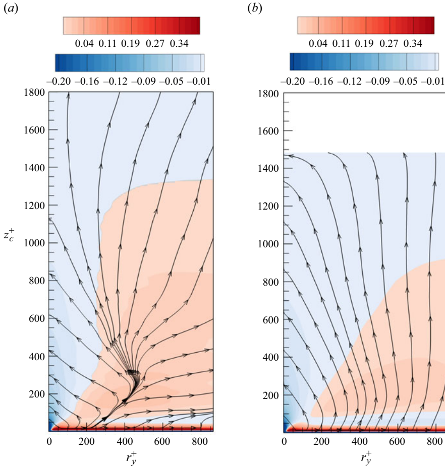
Figure 2. Fluxes of scale energy (black lines with arrows) in the compound space of spanwise scales and wall distances (\phi_{r_y}^+, \phi_{z_c}^+)(0, r_y^+, 0, z_c^+) and isocontours of the scale energy source \xi^+(0, r_y^+, 0, z_c^+) for a turbulent boundary layer (a) and a turbulent channel (b) at Re_\tau = 1500 .
