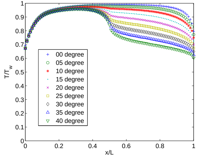
Fig. 12. Mean temperature along the channel, second-half divergent microchannel (case 3), for different divergent angles at a plenum pressure of 150 Pa and wall temperature of 573 K.
