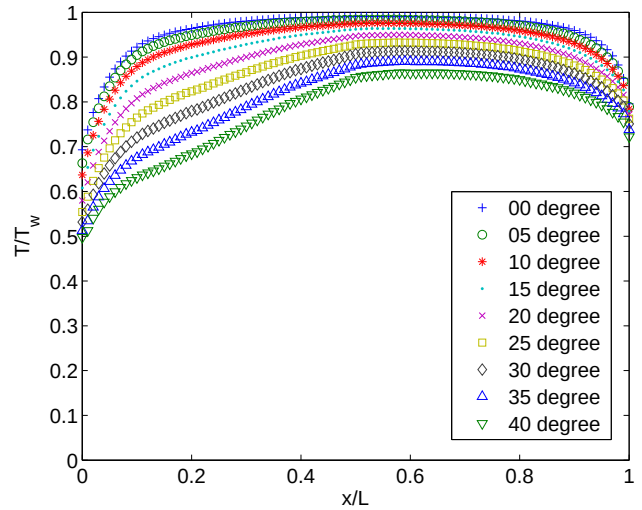
Fig. 16. Mean temperature along the channel, first-half divergent microchannel (case 4), for different divergent angles at a plenum pressure of 150 Pa and wall temperature of 573 K.
