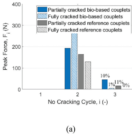
Figure 10. Effectiveness of bio-based couplets compared to reference couplets pre-cracked at 93 days: (a) peak force after multiple cracking-healing cycles with the relative healing ratio ( F_i/F_0 ) computed against the original capacity obtained at first cracking cycle; failure mode obtained in (b) self-healing and (c) control couplets at 158 days.
